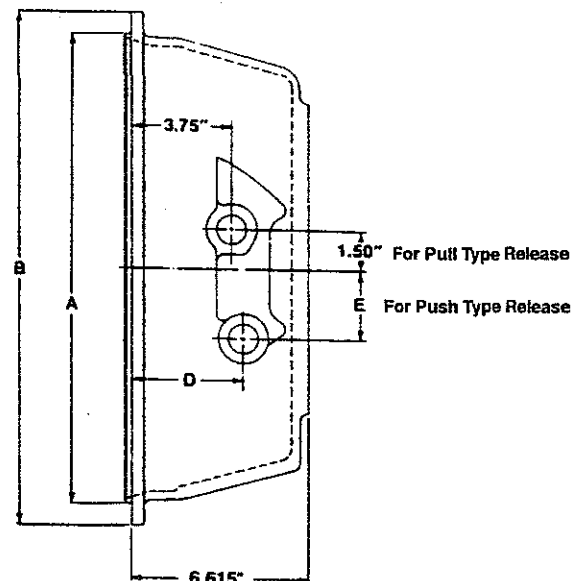
STANDARD MOUNT
