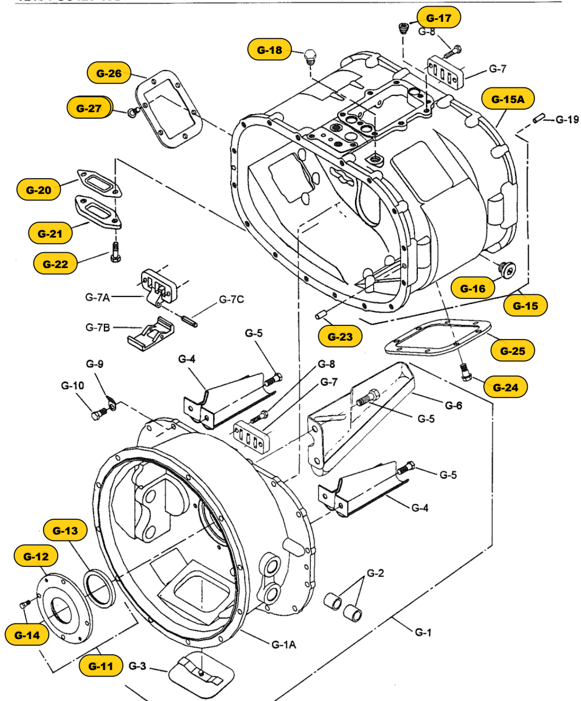
PRO-SHIFT 10 SPEED MODELS (1000-1350 lb-ft) CLUTCH HOUSING, FRONT BEARING CAP, and MAIN CASE T210-PSO125-10S
