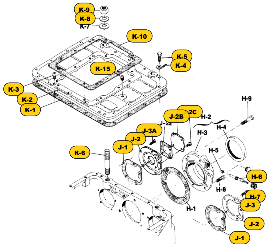
Rear Anchor Stud Chart
