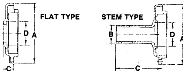
FRONT BEARING CAP CHART
