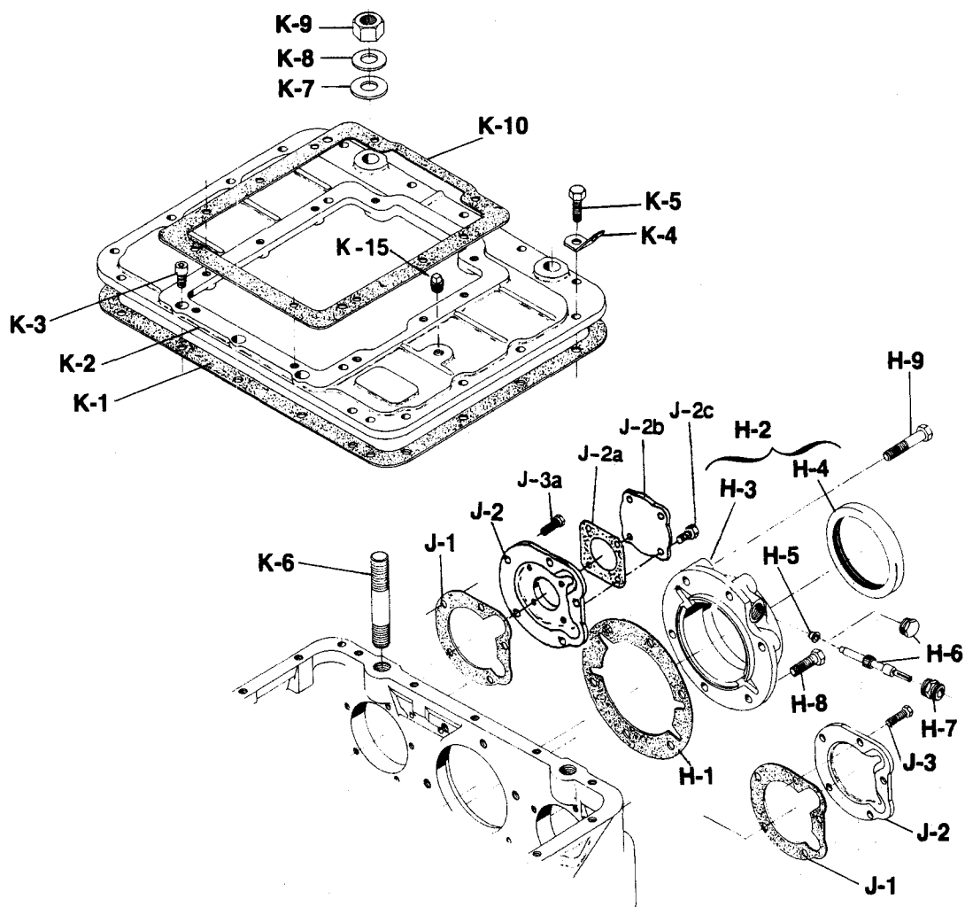
Rear Anchor Stud Chart
