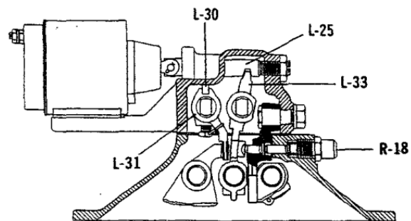
VIEW WITH SHIFT FINGERS ASSEMBLED
