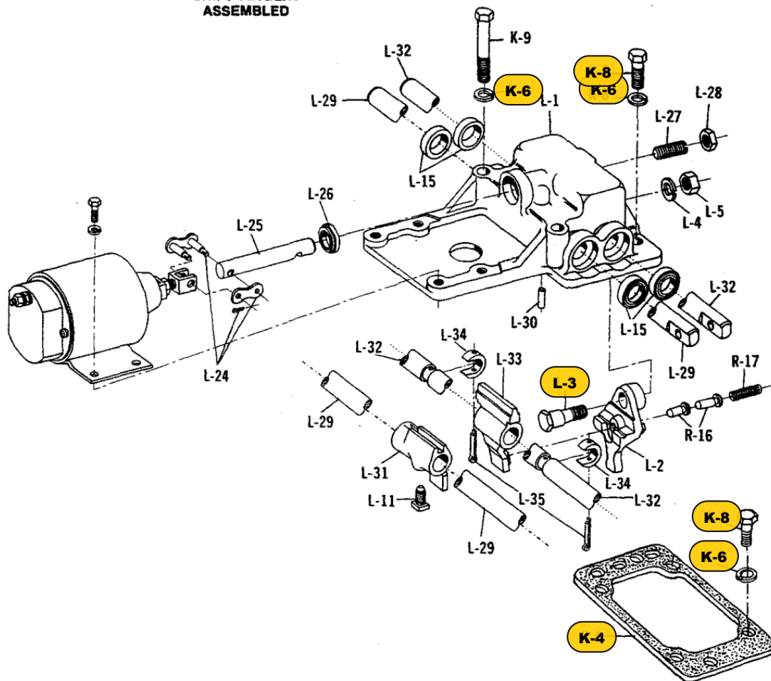
VIEW WITH SHIFT FINGERS ASSEMBLED
