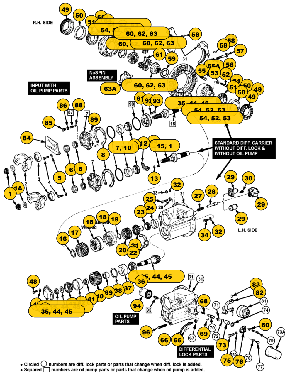
FIGURE 1 FORWARD CARRIERS OF TANDEM AXLES (USE WITH CHART 1)
