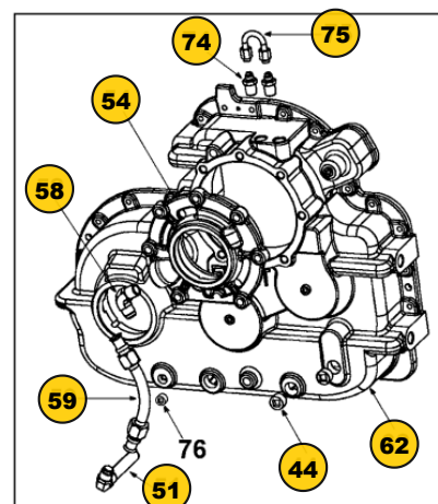
Oil Cooler Ready Components View
