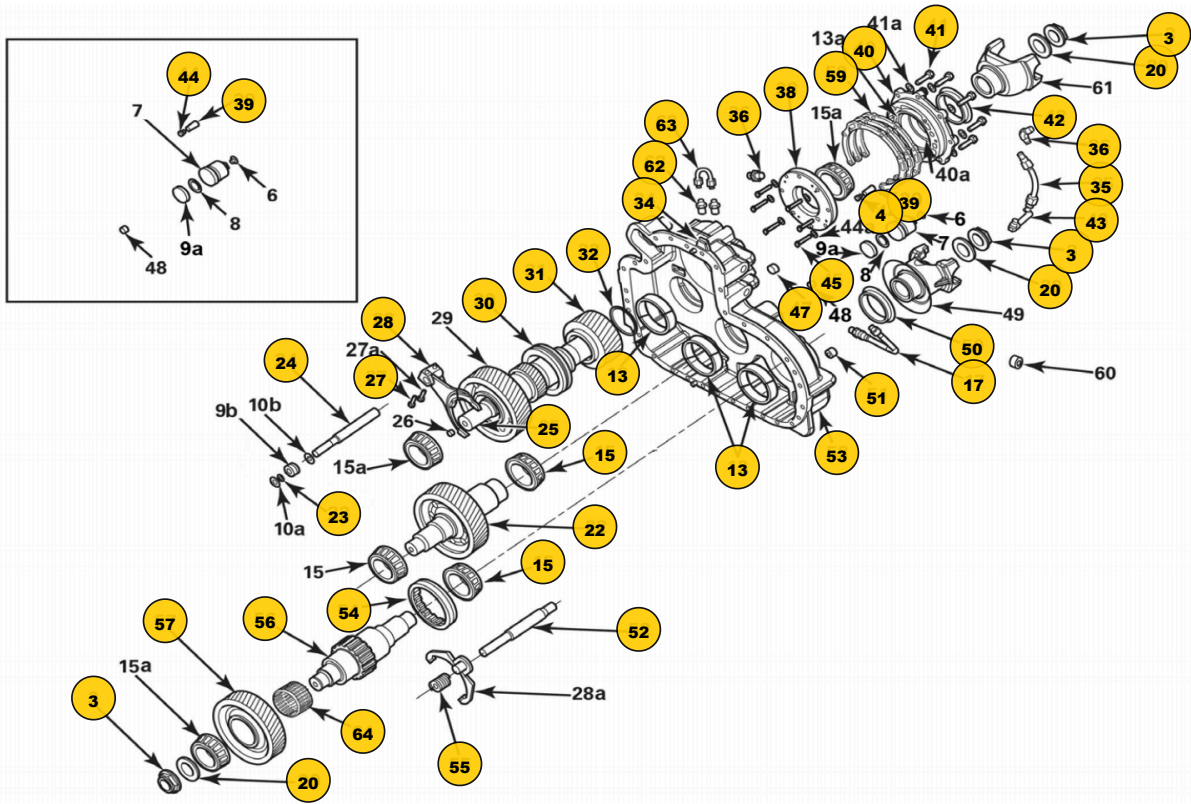
MTC4210 X / XP - Front
