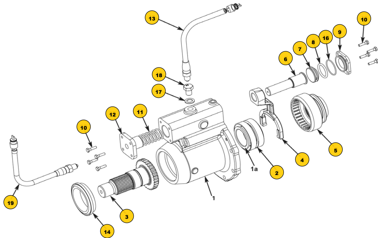
MTC4210 X / XP - PTO
