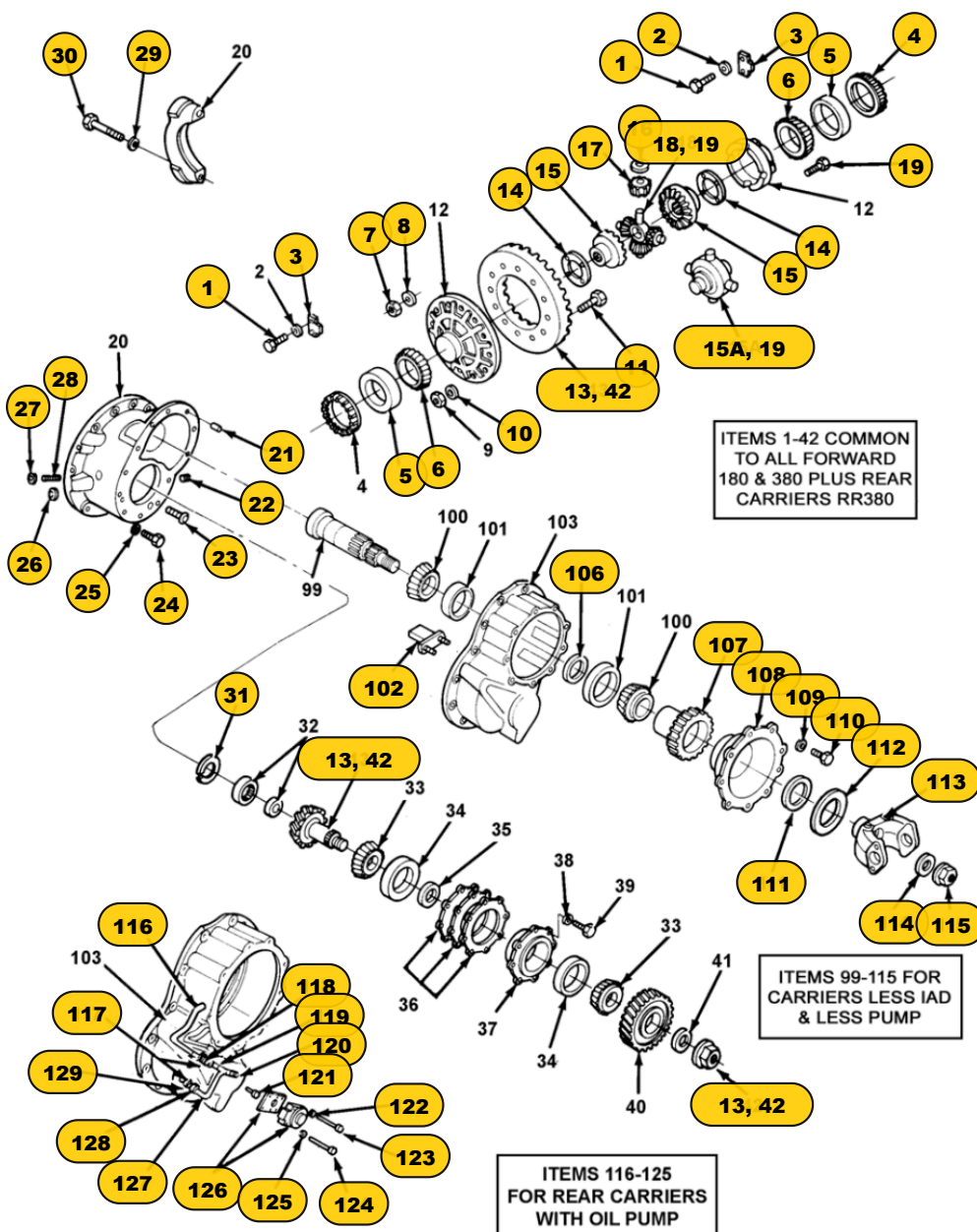
FIGURE 1 FORWARD CARIERS (180 & 380 LESS IAD & LESS PUMP) ALL REAR CARRIERS FOR 380 SERIES AXLES
