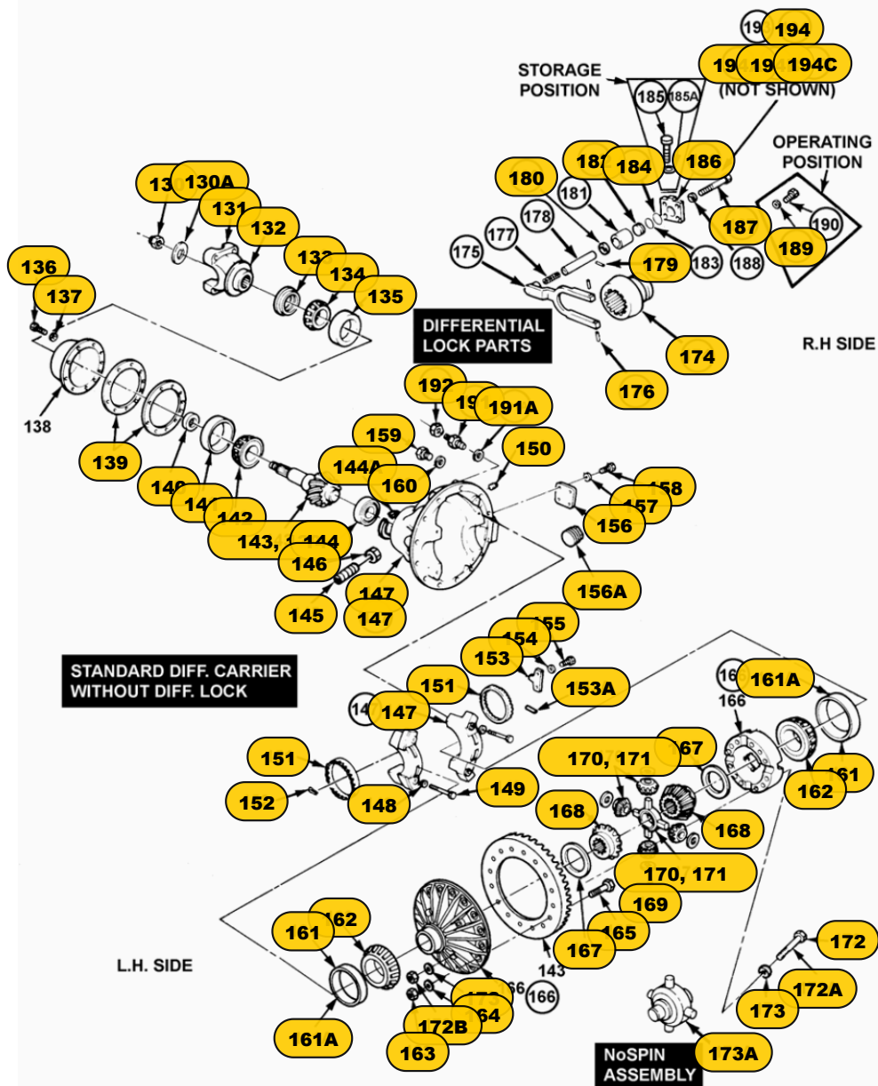
FIGURE 2 REAR CARRIERS FOR 180/185/186 SERIES SINGLE AND TANDEM AXLES
