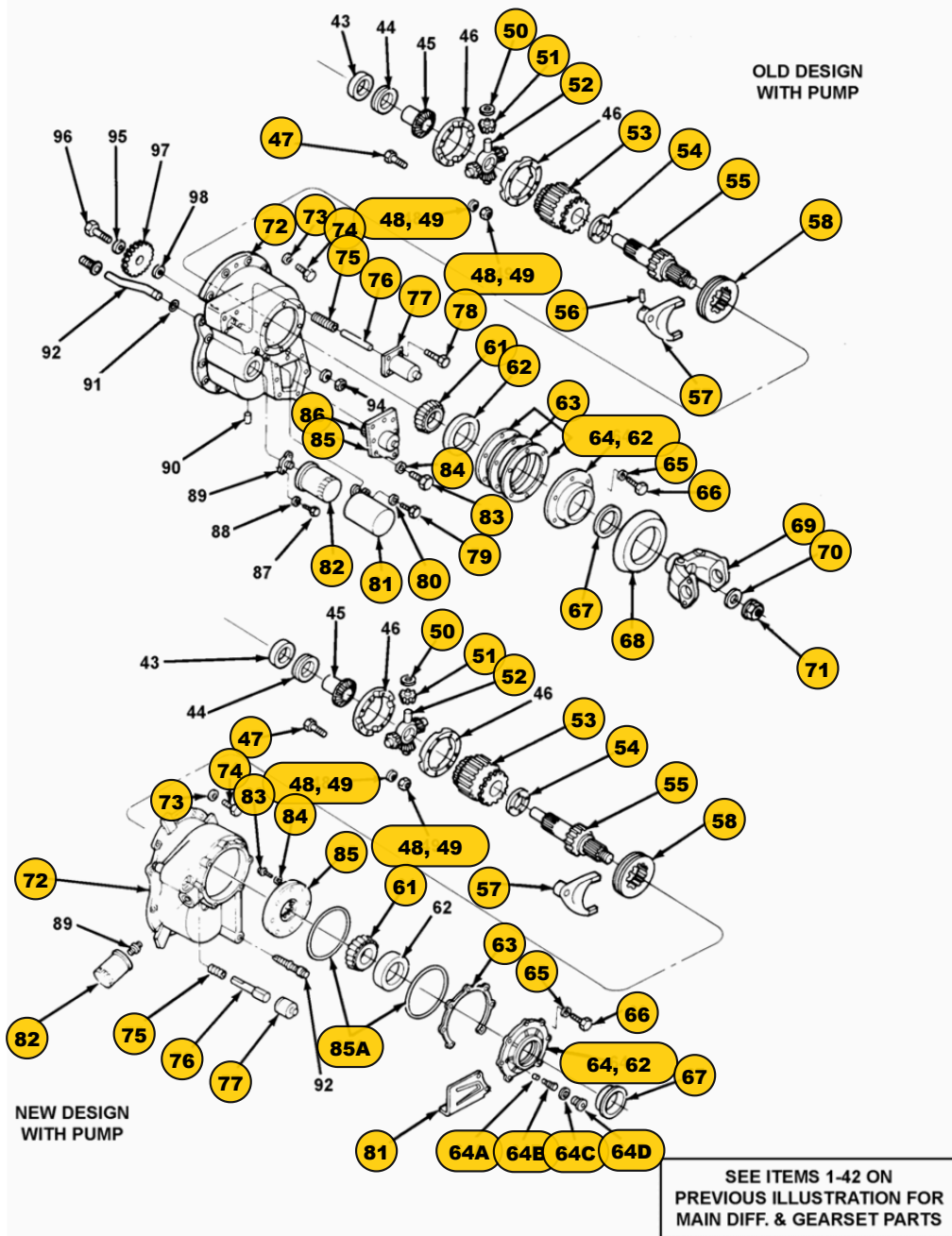
FIGURE 1A ALL FORWARD CARRIERS (180 & 380 WITH IAD & WITH PUMP)
