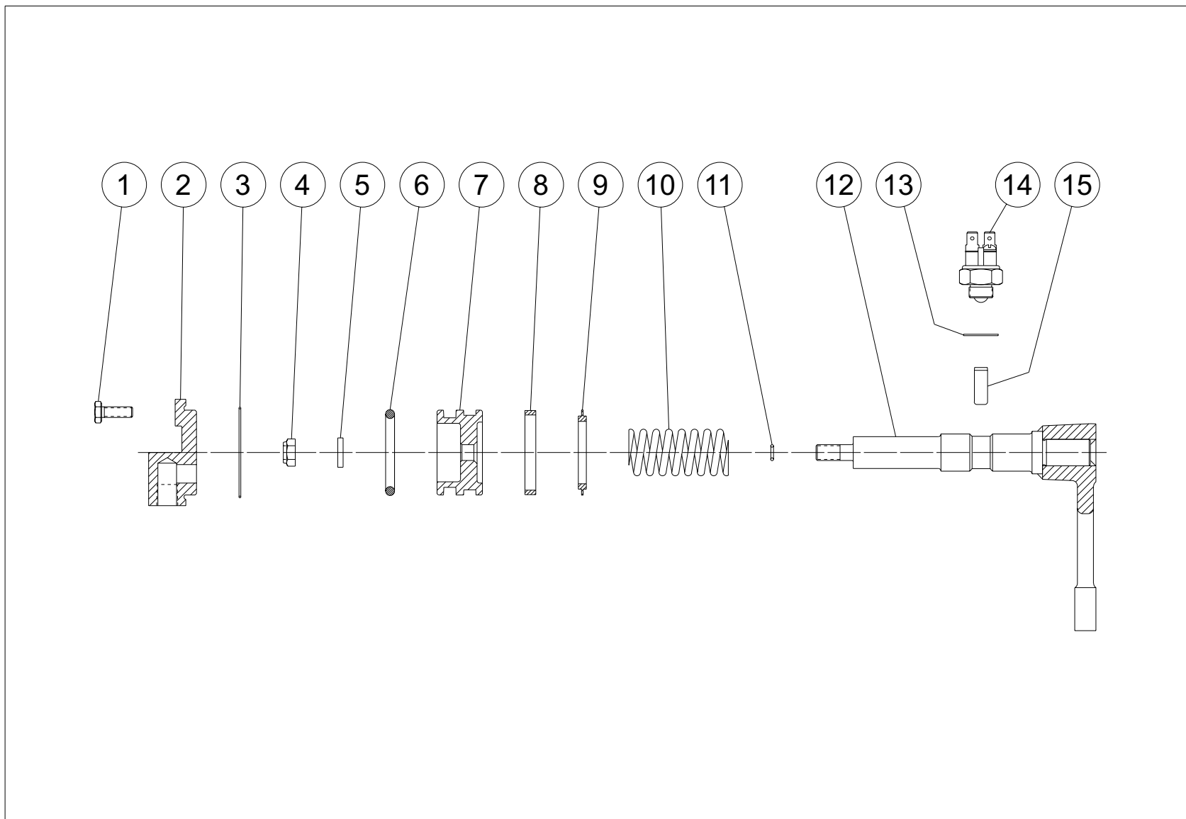
Figure P.6 - TC-200 Front Drive Shift Parts
