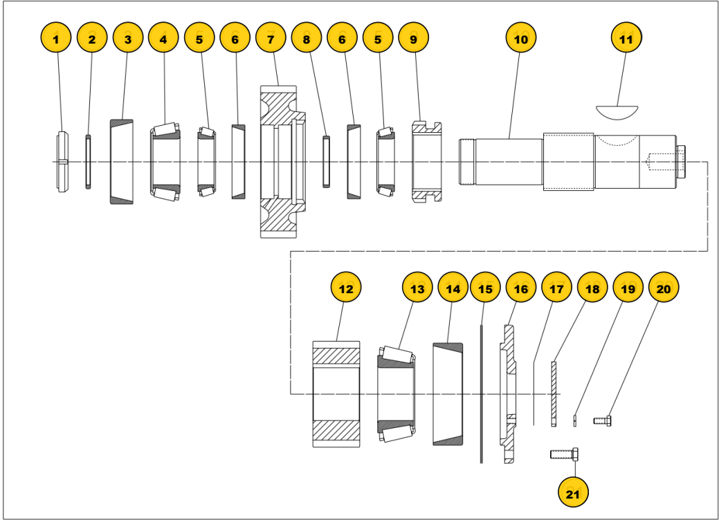
Figure P.3 - TC-200 Intermediate Shaft Parts
