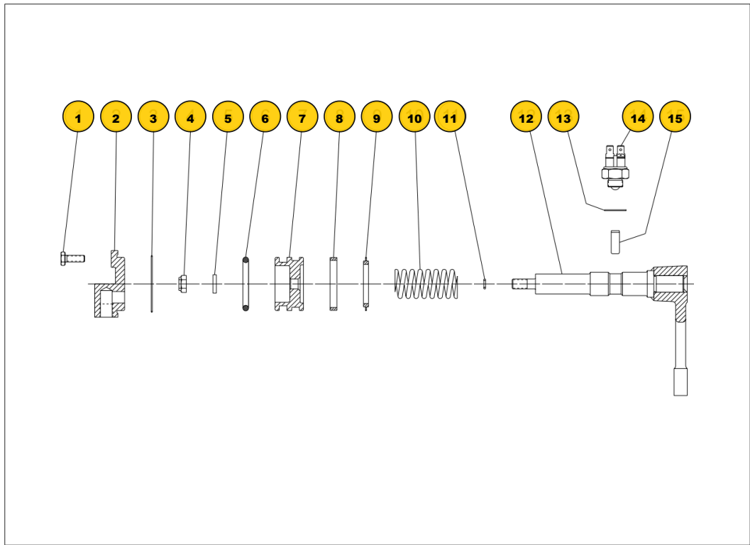
Figure P.6 - TC-200 Front Drive Shift Parts
