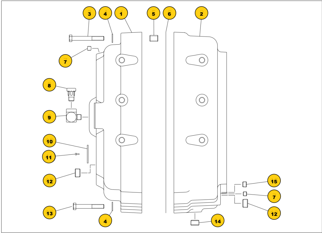
Figure P.9 - TC-200 Housing Parts
