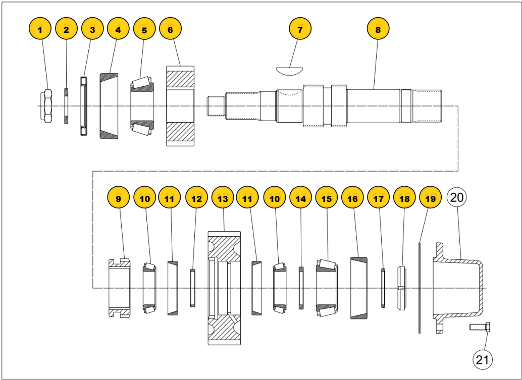
Figure P.2 - TC-200 Input Shaft Parts
