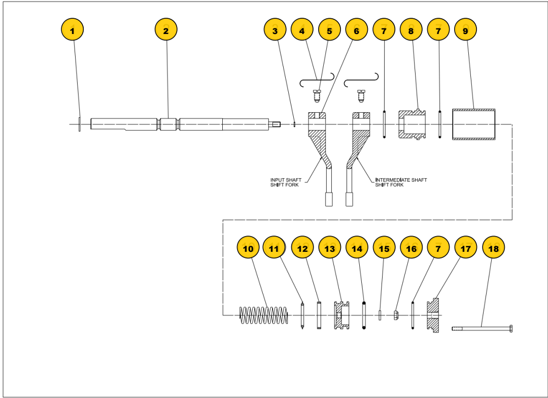
Figure P.7 - TC-200 High/Low Range Shift Parts
