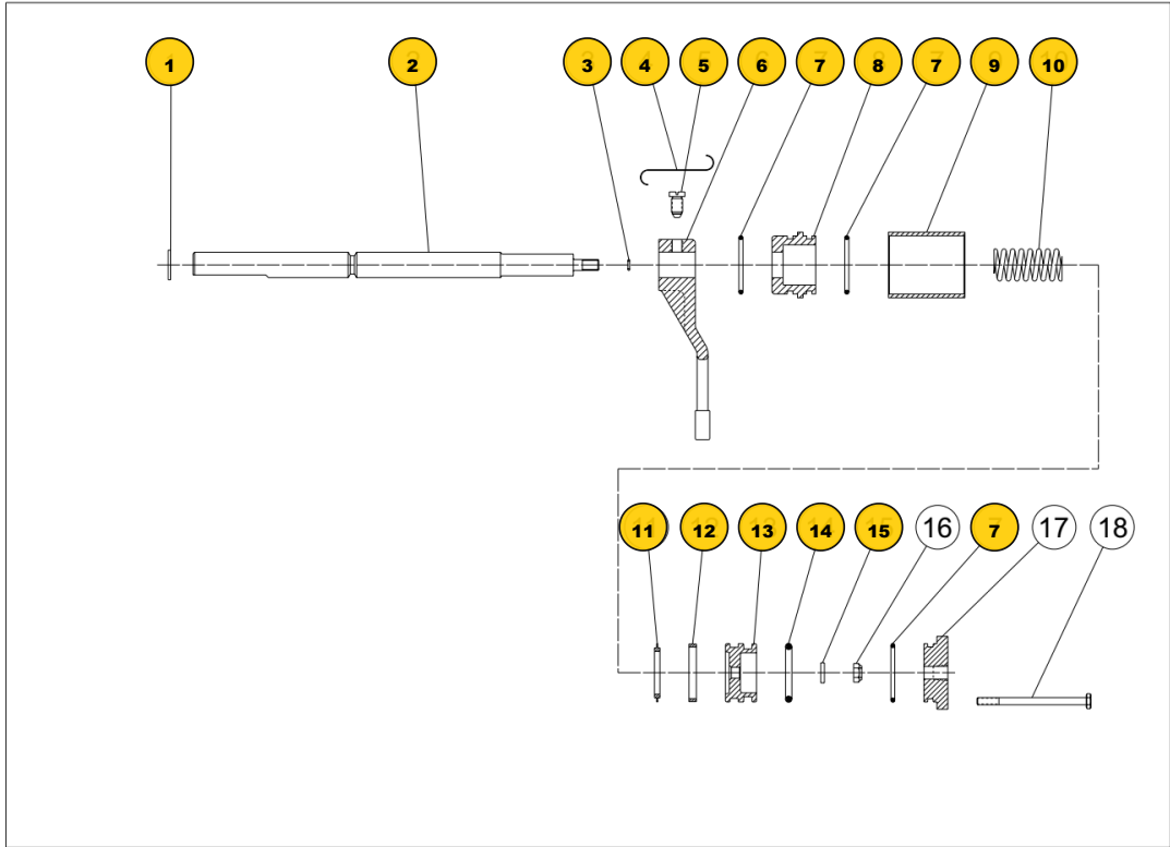
Figure P.8 - TC-200 Rear Drive Shift Parts
