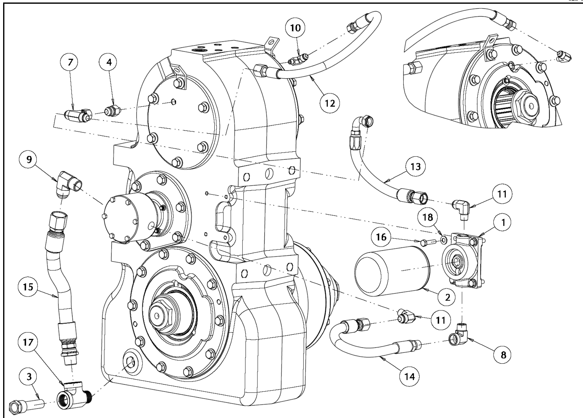
FIG. 12 - LUBRICATION AND FITTINGS
