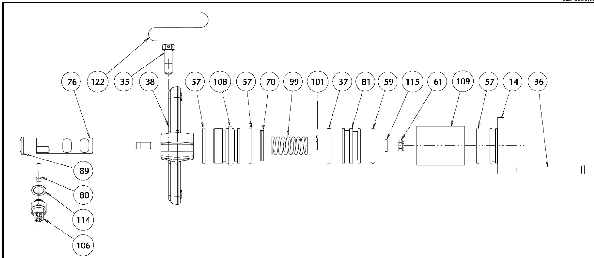
FIG. 11 - SINGLE-ACTING SHIFT CYLINDER ASSEMBLY All Models
