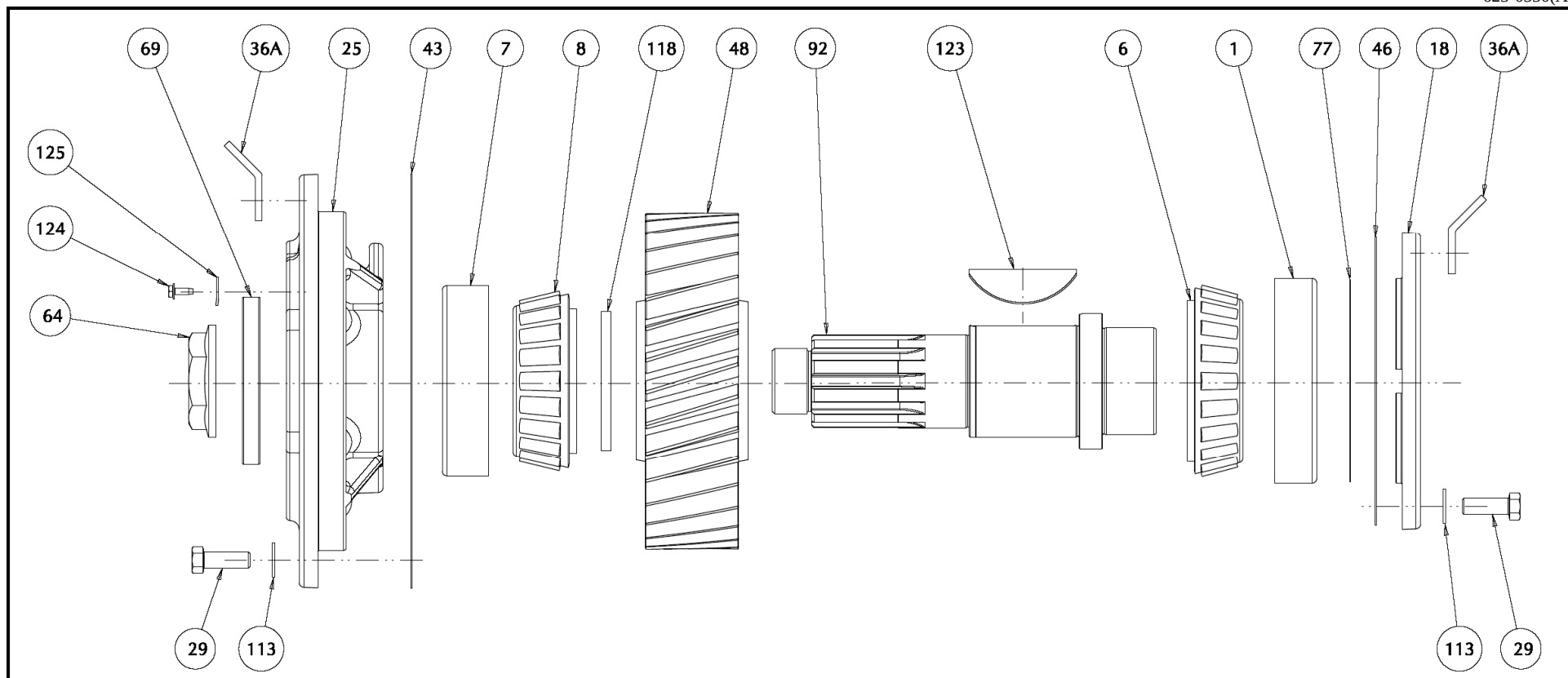
FIG. 4 - UPPER SHAFT ASSEMBLY Models without PTO Output
