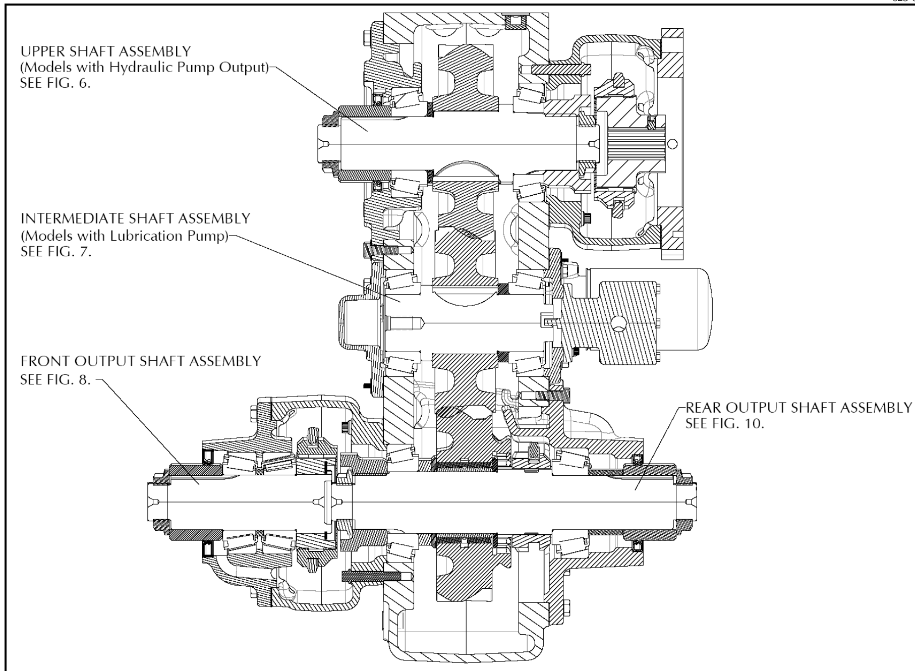
FIG. 3 - TYPICAL TC-180 BASIC TRANSFER CASE
