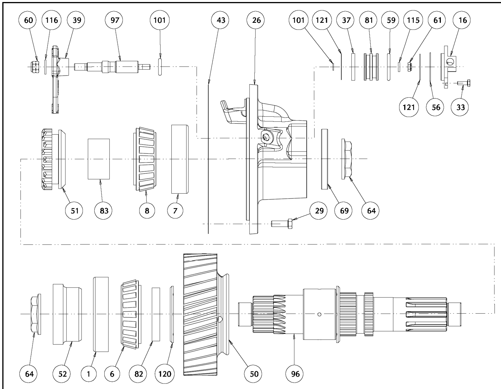
FIG. 10 - REAR OUTPUT SHAFT ASSEMBLY
