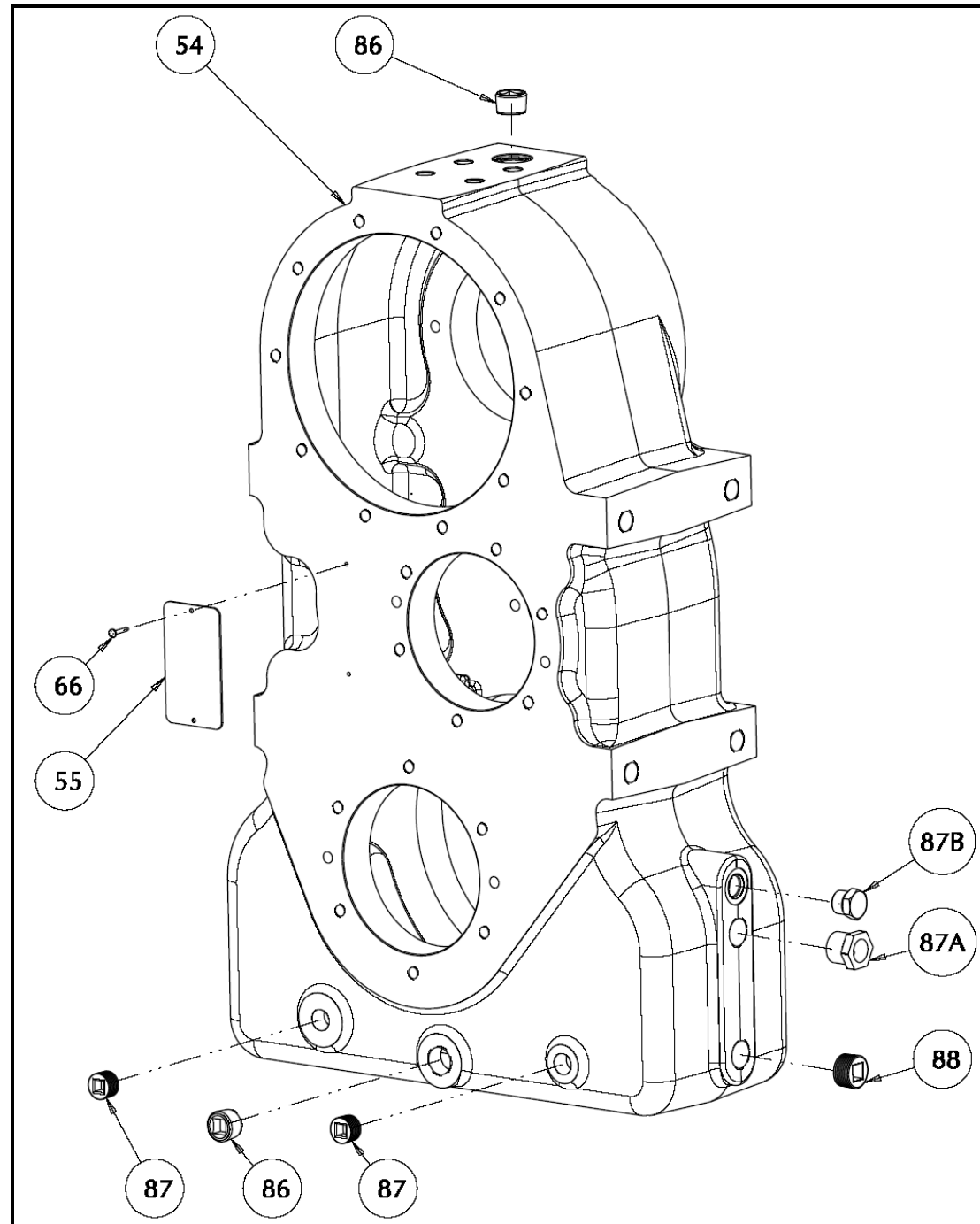
FIG. 14 - REMAINING PARTS
