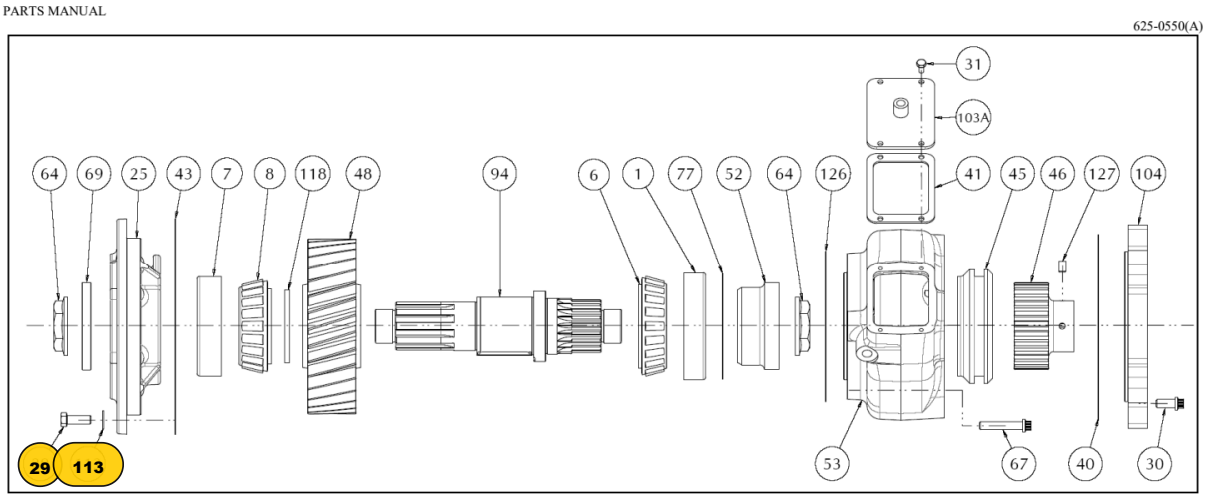
FIG. 6 - UPPER SHAFT ASSEMBLY Models with Hydraulic Pump Output
