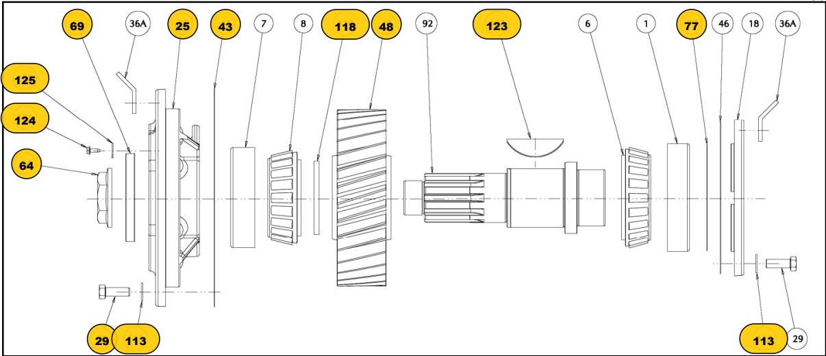
FIG. 4 - UPPER SHAFT ASSEMBLY Models without PTO Output
