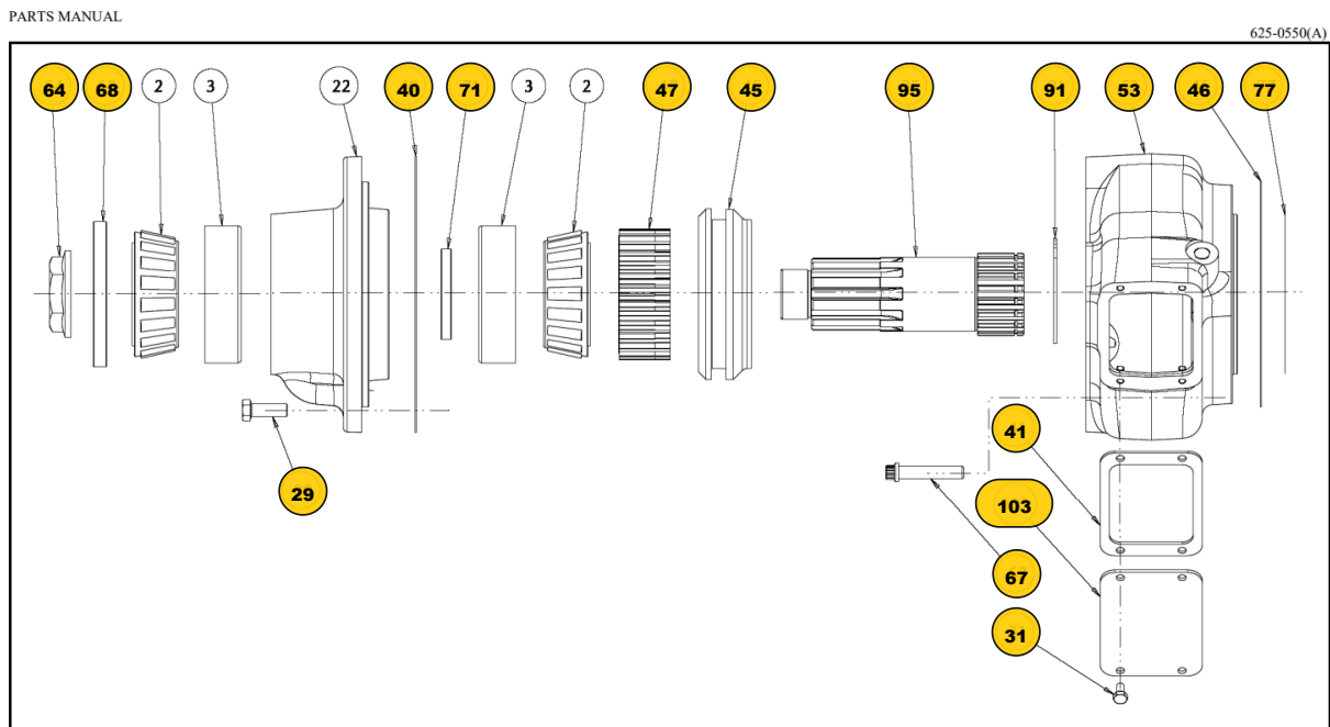
FIG. 8 - FRONT OUTPUT SHAFT ASSEMBLY
