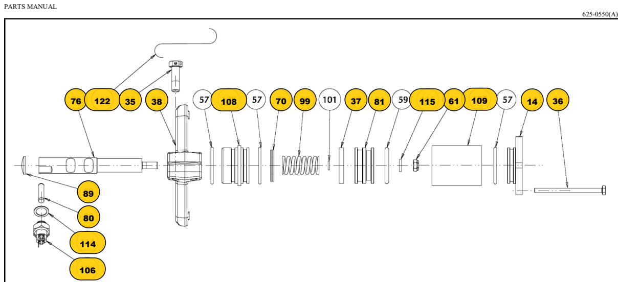
FIG. 11 - SINGLE-ACTING SHIFT CYLINDER ASSEMBLY All Models
