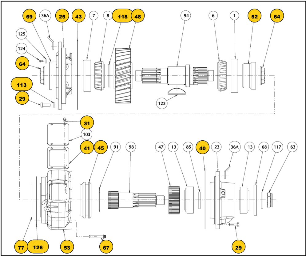
FIG. 5 - UPPER SHAFT ASSEMBLY
