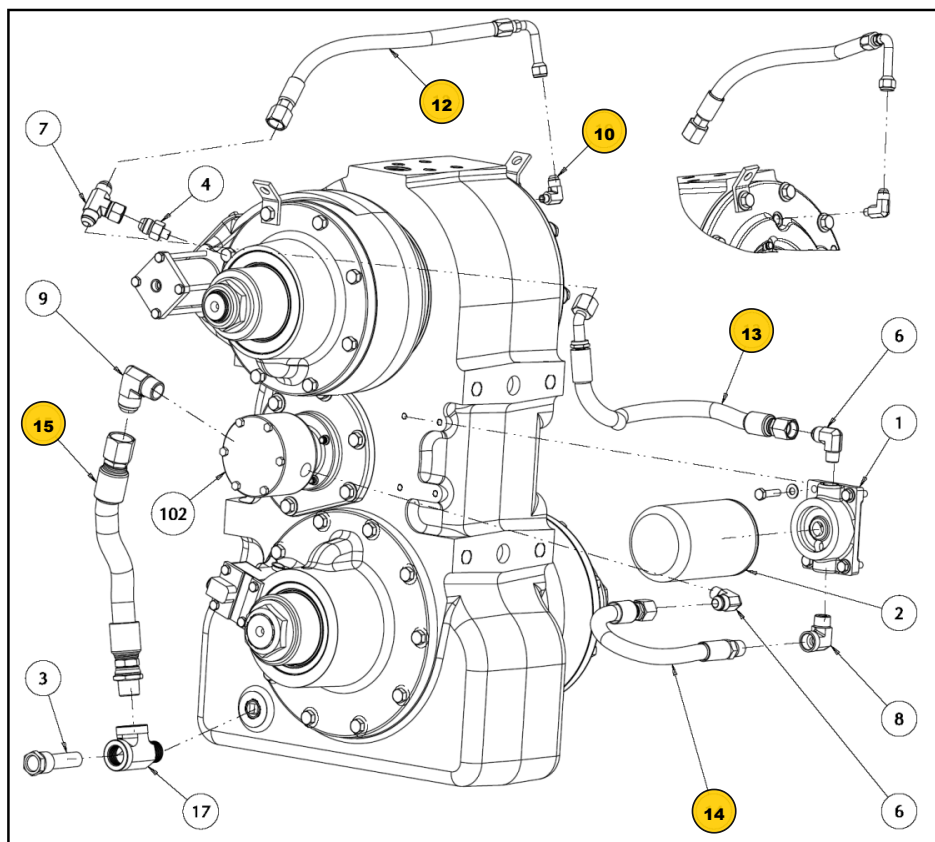
FIG. 13 - LUBRICATION AND FITTINGS
