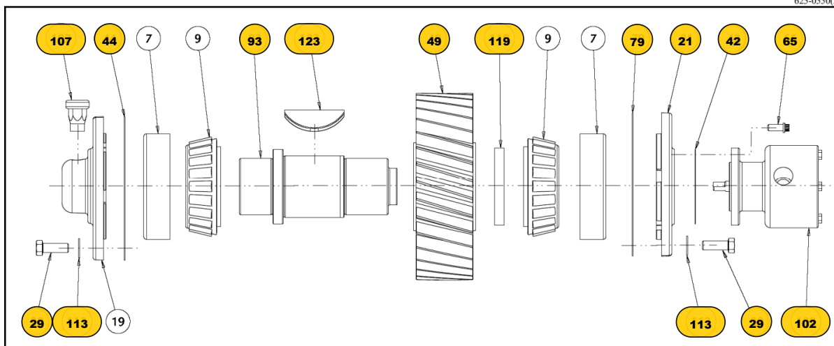
FIG. 7 - INTERMEDIATE SHAFT ASSEMBLY
