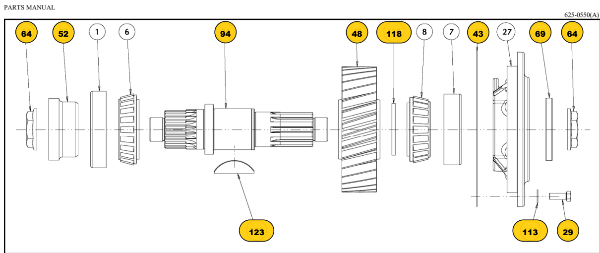
FIG. 9 - REAR OUTPUT SHAFT ASSEMBLY Models without Neutral
