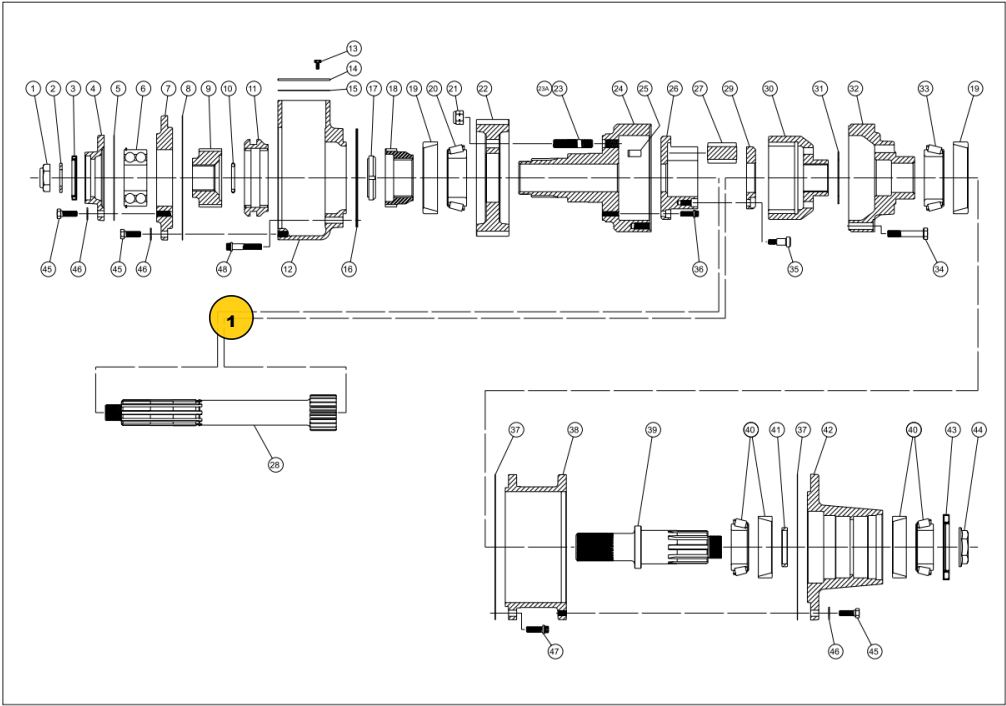
FIG P.13 - TC-170 PD 33/67 LOWER SHAFT ASSEMBLY
