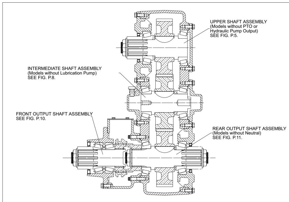
FIG P.1 - TYPICAL TC-170 BASIC TRANSFER CASE
