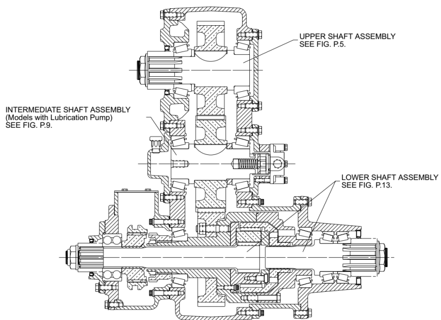
FIG P.3 - TYPICAL TC-170 P.D. TRANSFER CASE (with 33/67 PROPORTIONAL DIFFERENTIAL)
