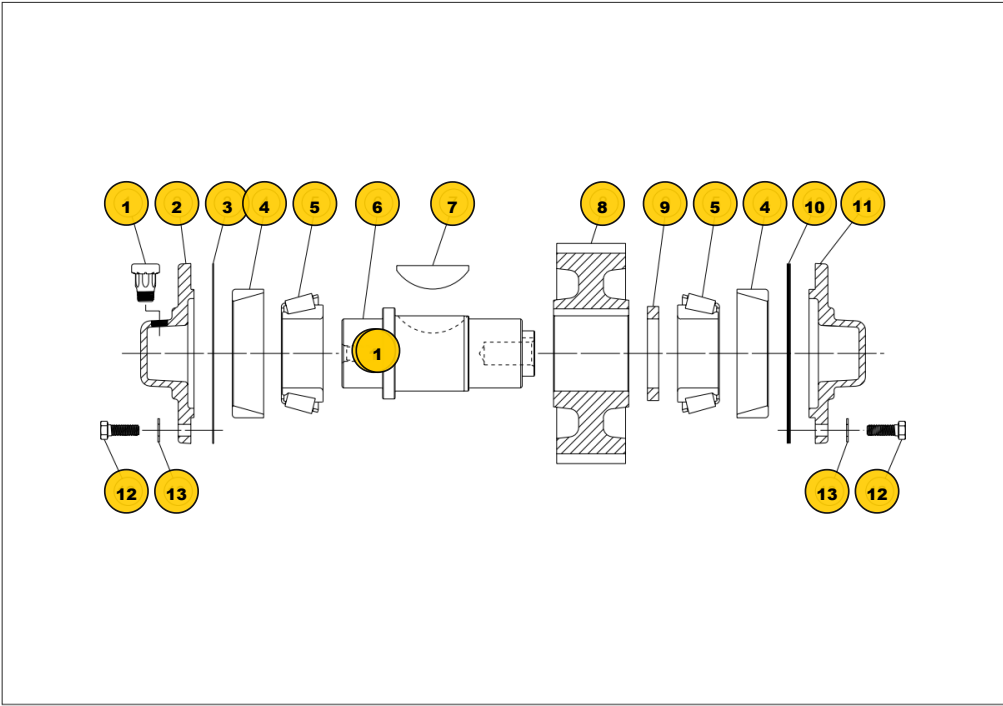
FIG P.8 - INTERMEDIATE SHAFT ASSEMBLY Models without Lubrication Pump
