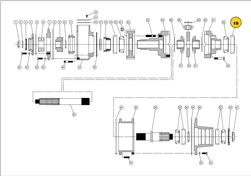
FIG P.14 - TC-170 PD 50/50 LOWER SHAFT ASSEMBLY
