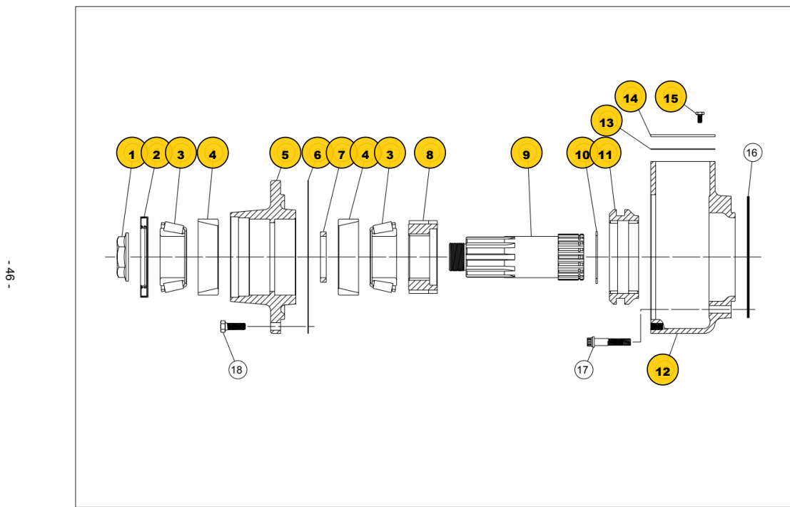
FIG P.10 - FRONT OUTPUT SHAFT ASSEMBLY Basic Transfer Cases (without Proportional Differential)
