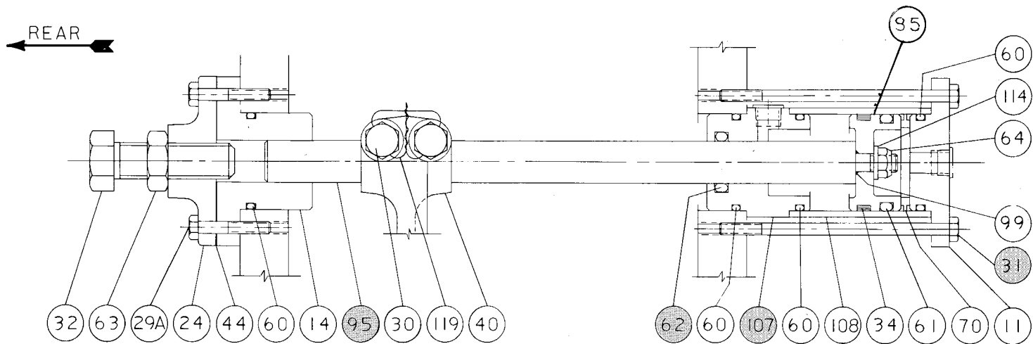
POWER TAKE OFF SHIFT DETAILS
