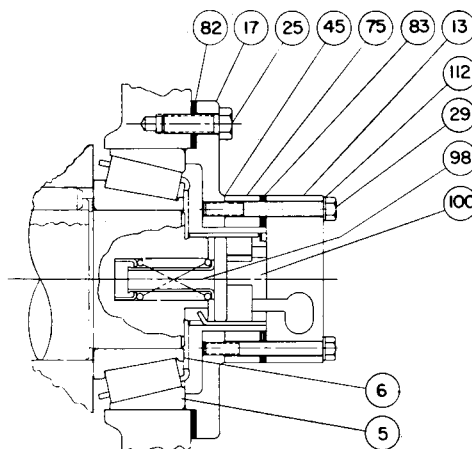
OPTIONAL LUBRICATION PUMP
