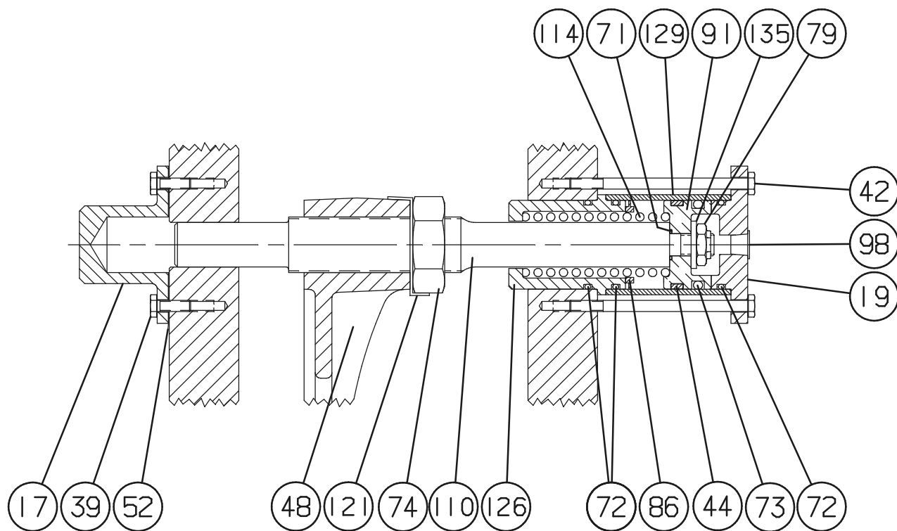
SINGLE ACTING SHIFT CYLINDER
