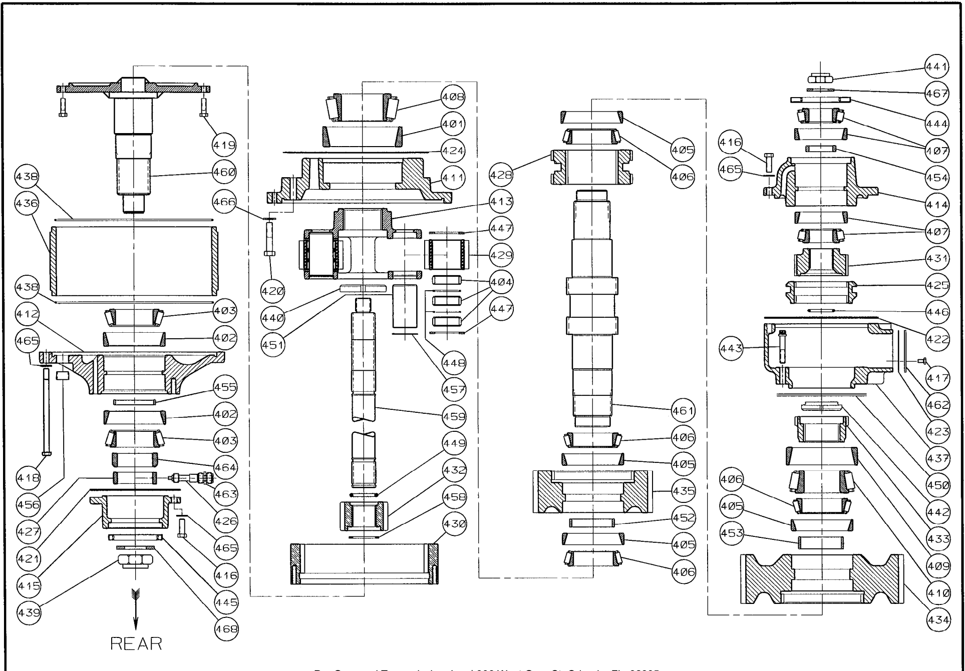
FIGURE 8.3 TC-142 PD LOWER SHAFT PARTS
