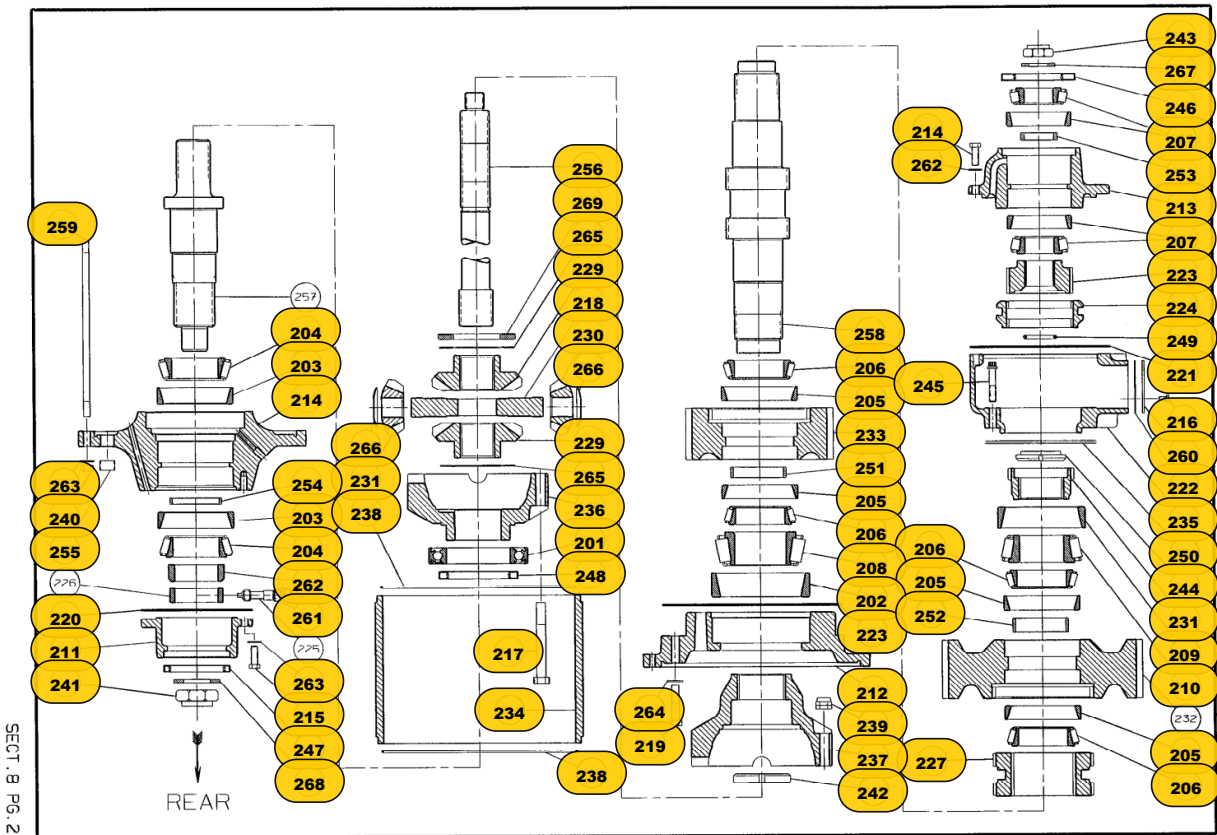
FIGURE 8-1 TC-142PD 50/50 LOWER SHAFT PARTS
