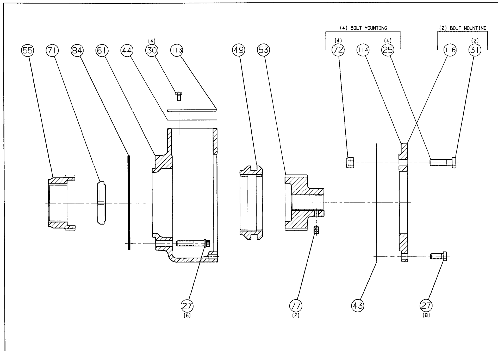
FIGURE 8.8 , TC-142 &amp; TC-1421 , HYDRAULIC PUMP DRIVE MOUNTING PARTS
