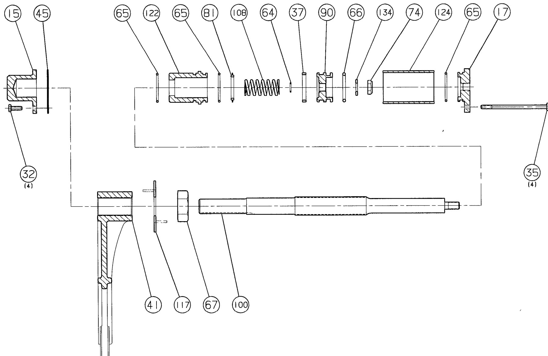
FIGURE 8.12 , TC-1421 , AIR SHIFT CYLINDER PARTS FOR DIRECT &amp; NEUTRAL
