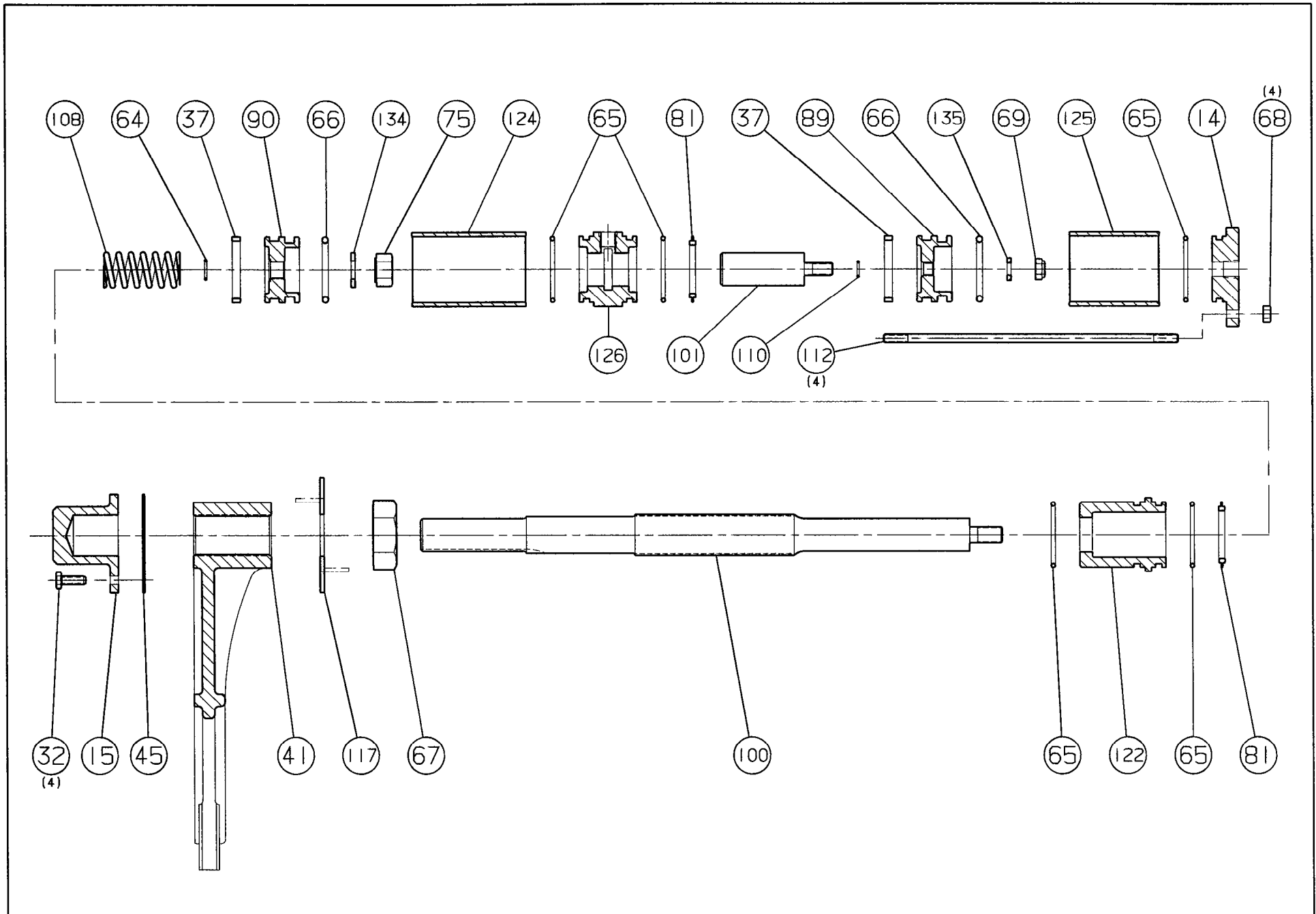
FIGURE 8.11 , TC-142 , AIR SHIFT CYLINDER PARTS FOR DIRECT , NEUTRAL &amp; UNDERDRIVE
