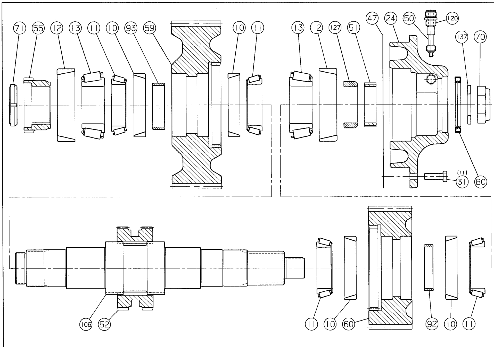
FIGURE 8.4 TC-142 LOWER SHAFT PARTS
