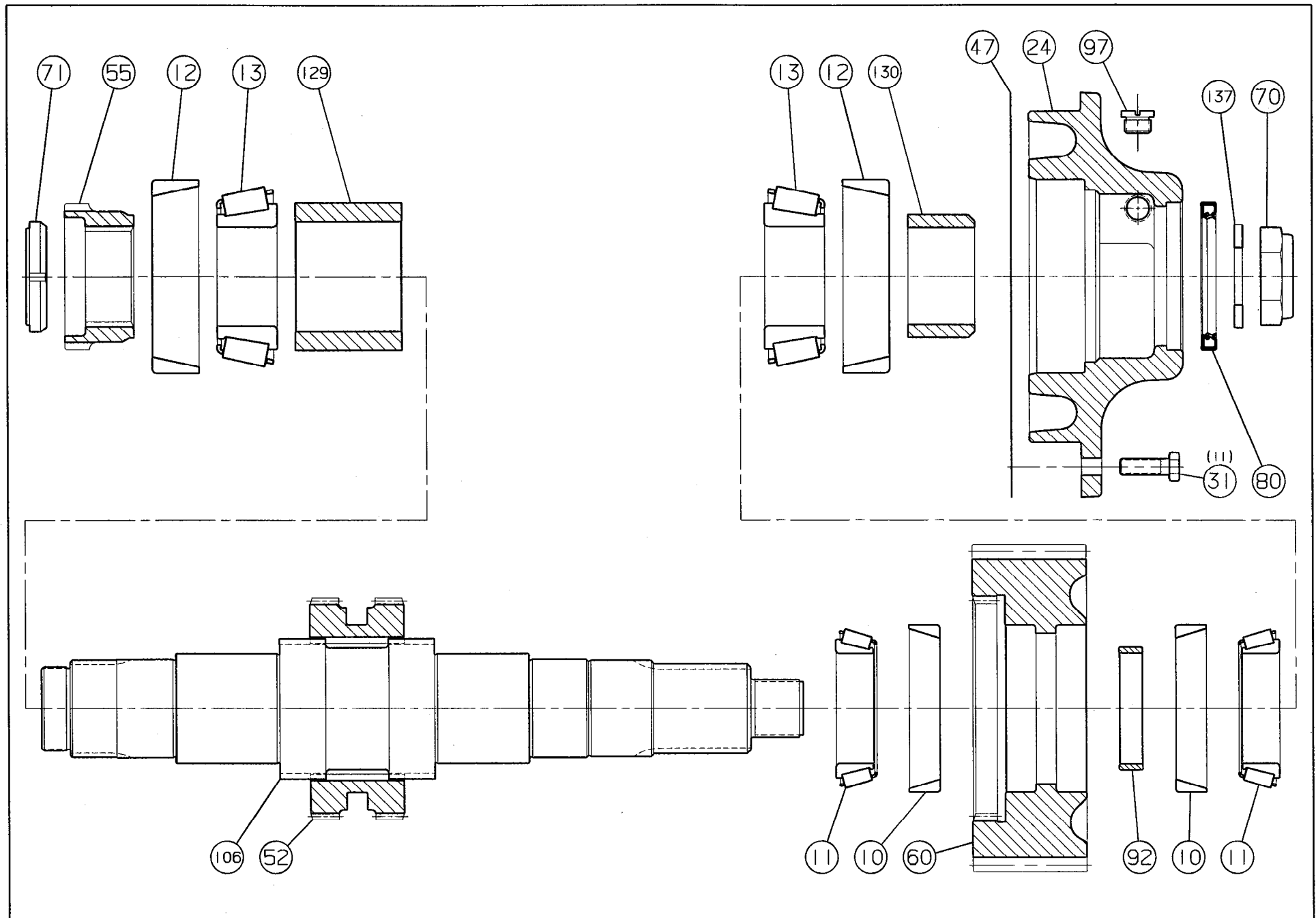
FIGURE 8.5 TC-142 LOWER SHAFT PARTS
