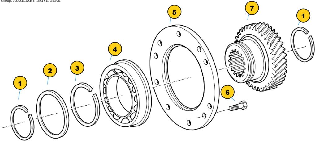
Group: AUXILIARY DRIVE GEAR
