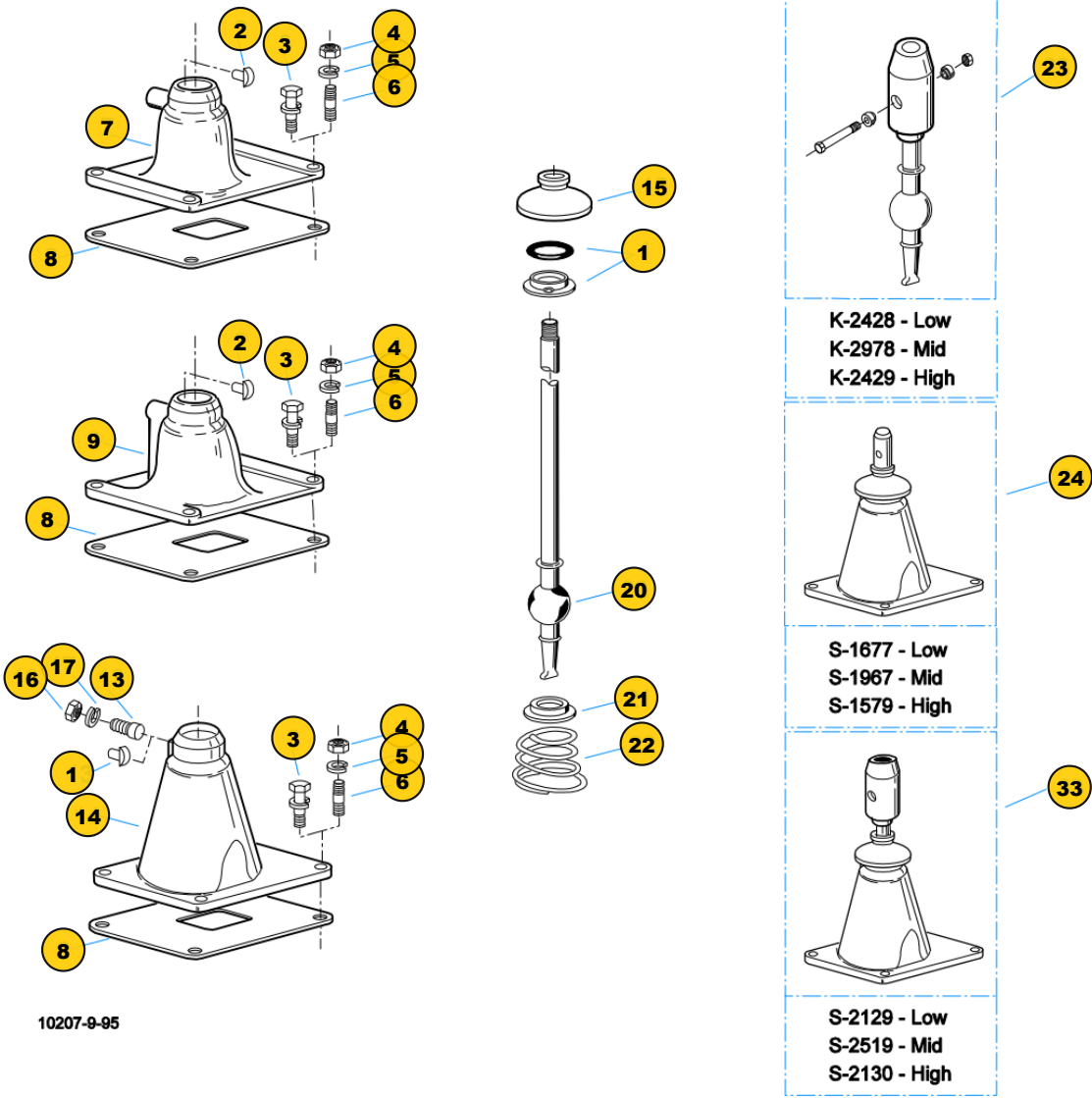
Group: LEVERS/HOUSINGS
