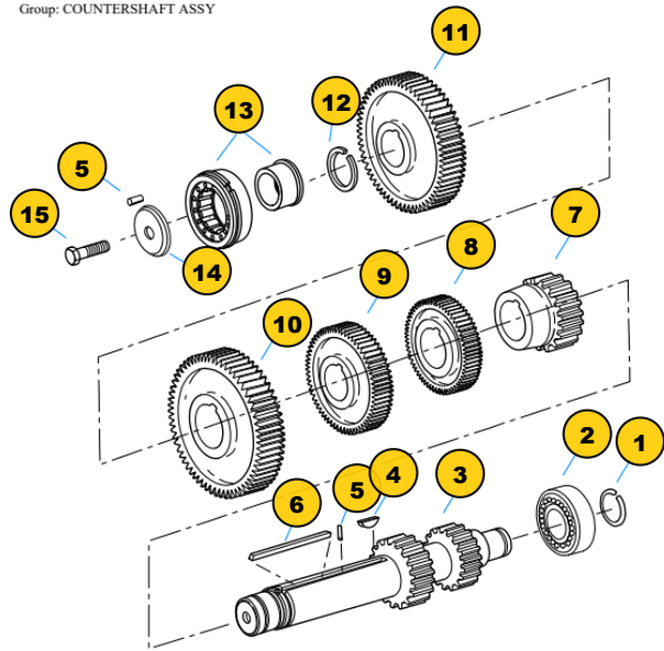
Group: COUNTERSHAFT ASSY
