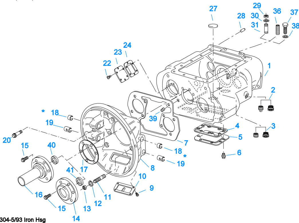
10304-5/93 Iron Hsg
