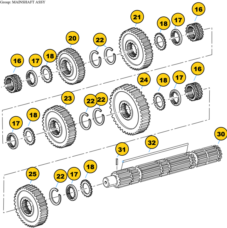
Group: MAINSHAFT ASSY
