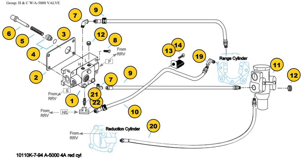
Group: H & C W/A-5000 VALVE
