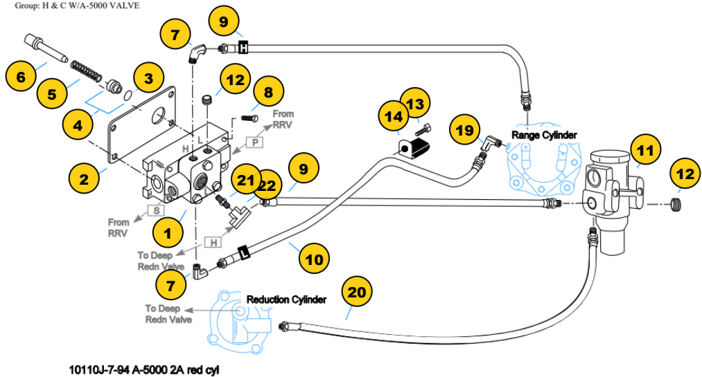
Group: H & C W/A-5000 VALVE
