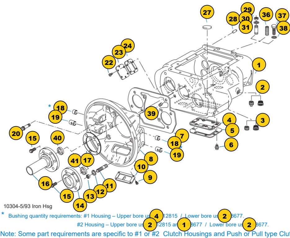
Group: CASE (FRONT)
