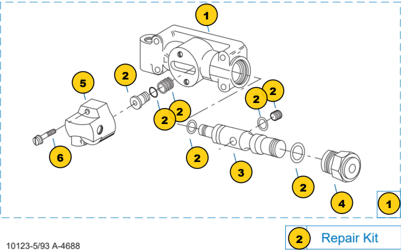
Group: SLAVE VALVE - A-4688
