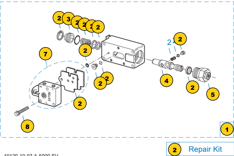
Group: SLAVE VALVE - A-5000
