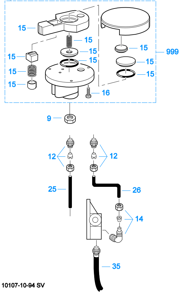
Group: SELECTOR VALVE ASSY
