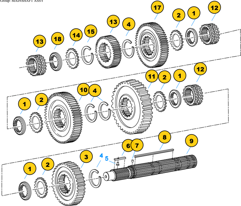
Group: MAINSHAFT ASSY
