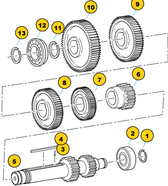
Group: COUNTERSHAFT ASSY
