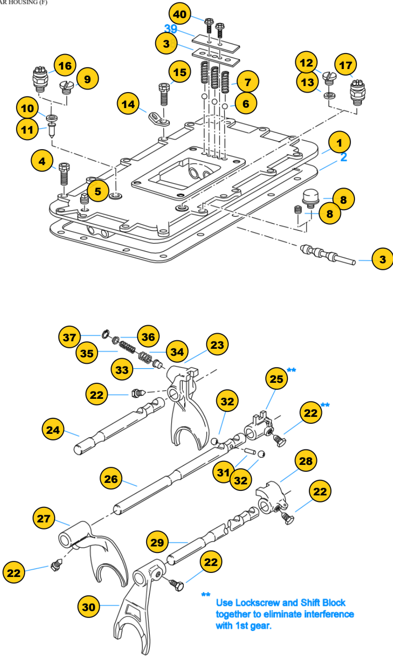
Group: SHIFT BAR HOUSING (F)
