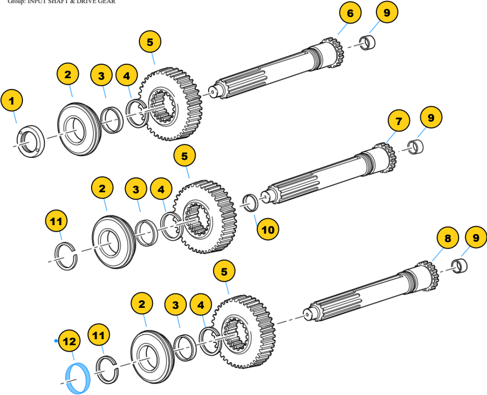
Group: INPUT SHAFT & DRIVE GEAR
