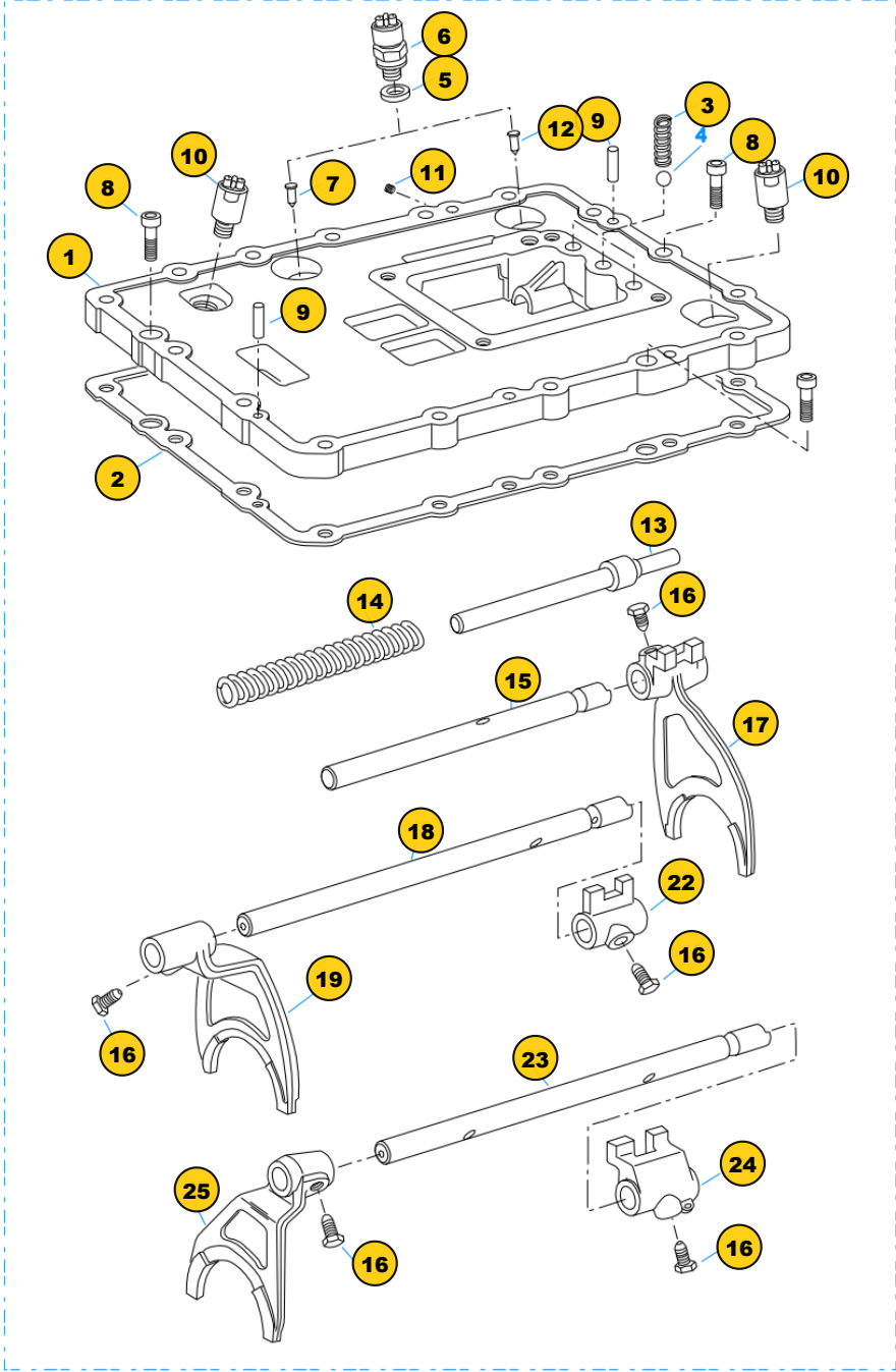
Group: BAR HOUSING ASSY
