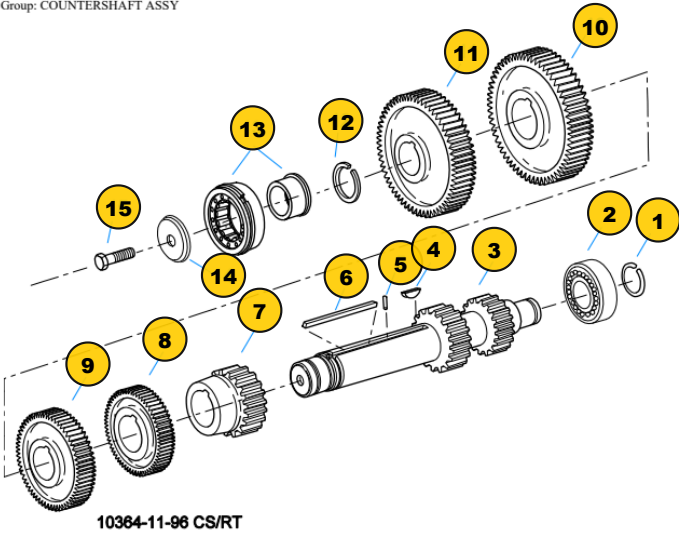
Group: COUNTERSHAFT ASSY
