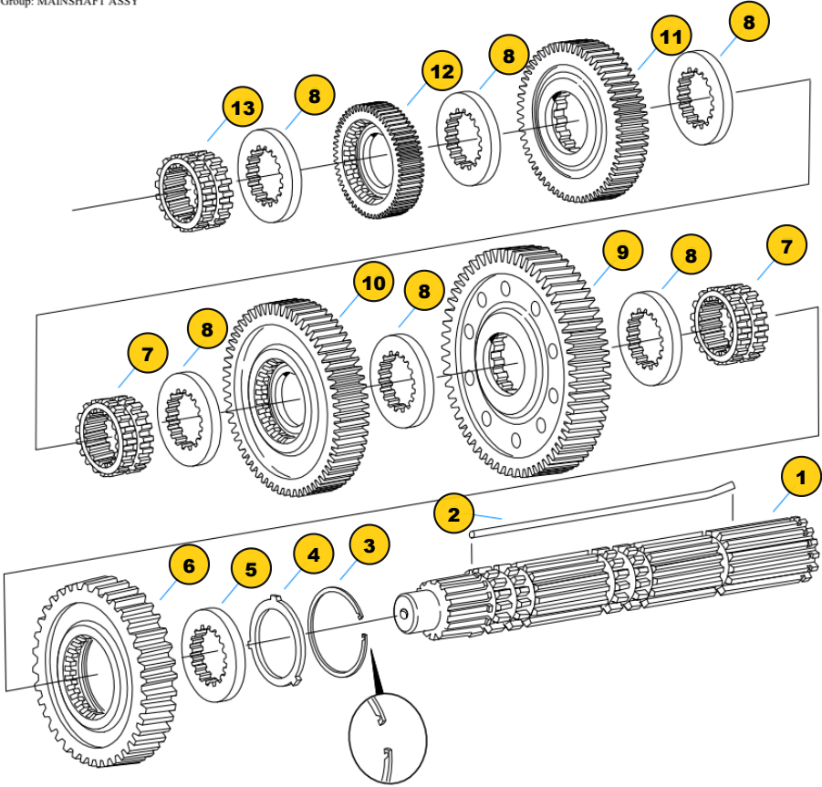
Group: MAINSHAFT ASSY
