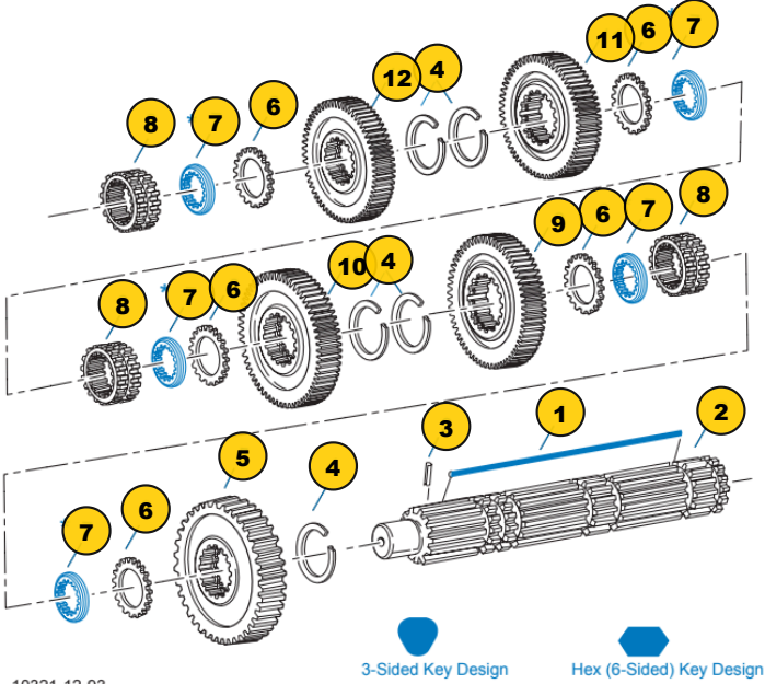
Group: MAINSHAFT ASSY
