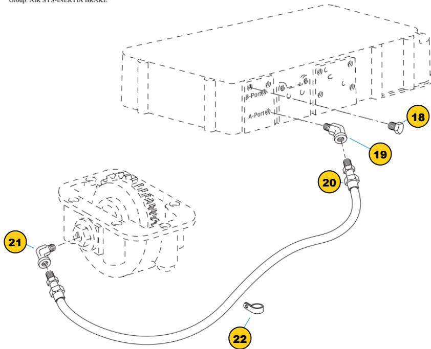
Group: AIR SYS-INERTIA BRAKE
