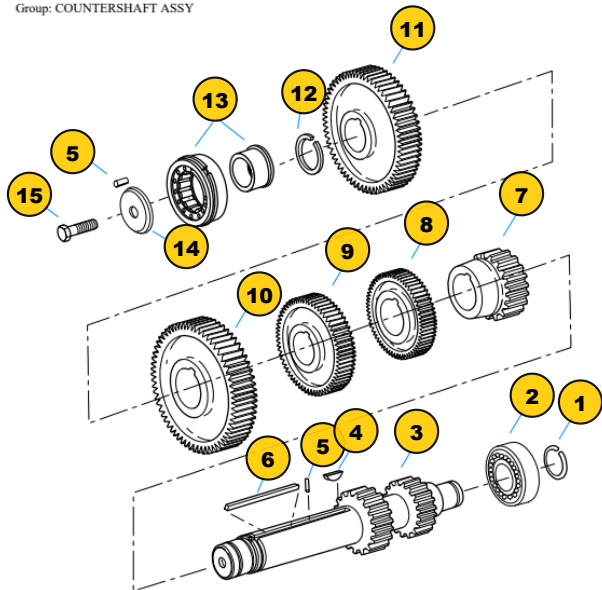
Group: COUNTERSHAFT ASSY
