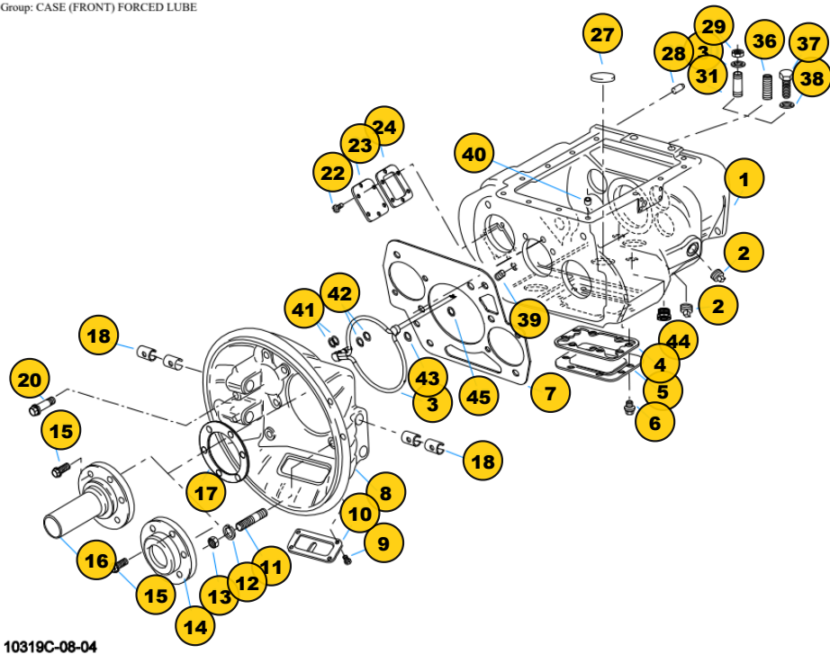
Group: CASE (FRONT) FORCED LUBE
