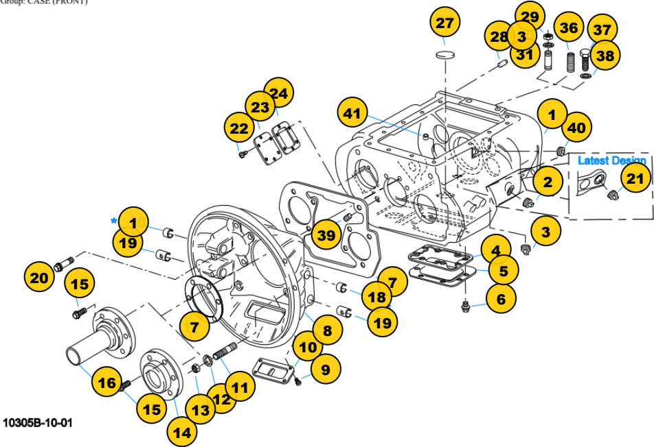
Group: CASE (FRONT)
