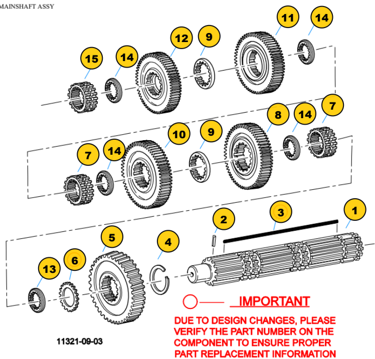
Group: MAINSHAFT ASSY
