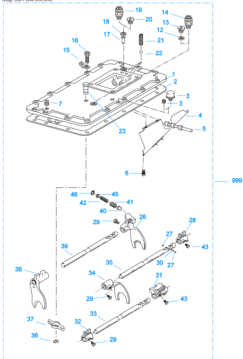
10241-3-94 X-Bar
