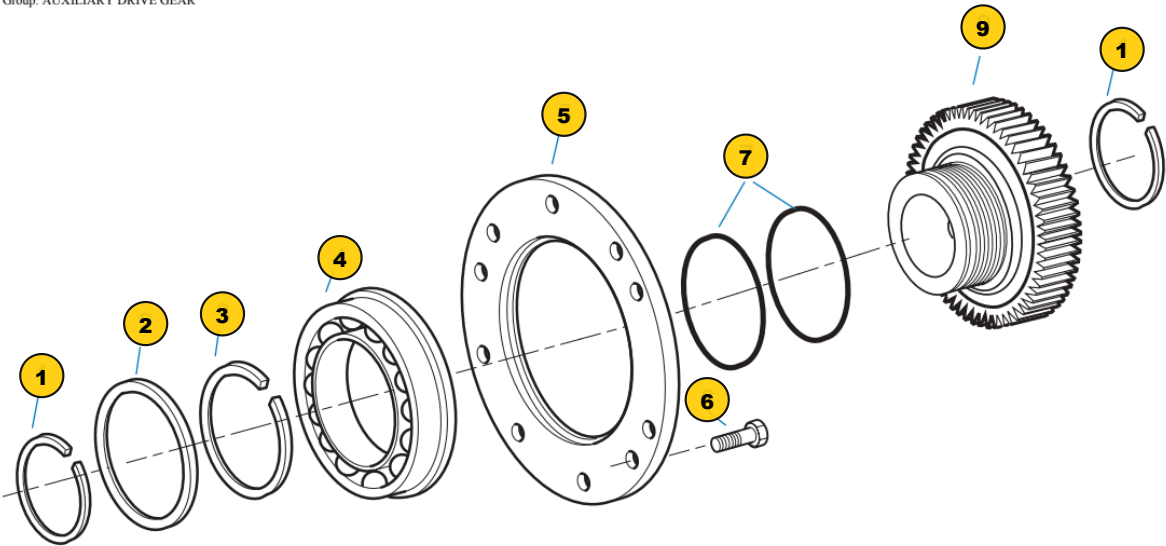
Group: AUXILIARY DRIVE GEAR
