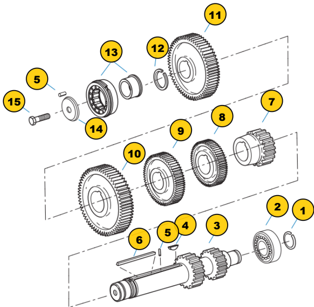
Group: COUNTERSHAFT ASSY
