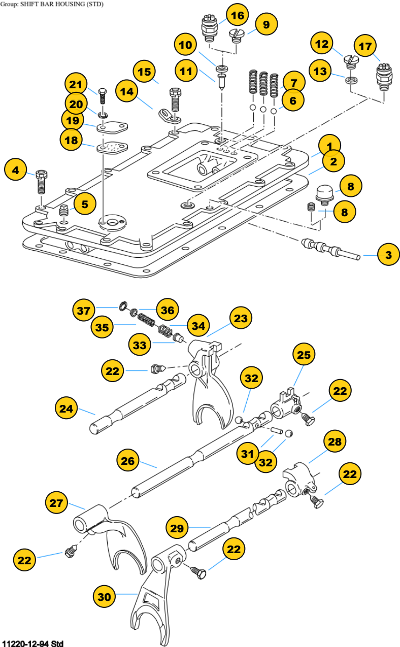
Group: SHIFT BAR HOUSING (STD)
