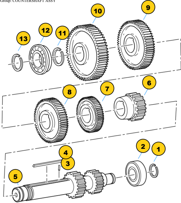
Group: COUNTERSHAFT ASSY
