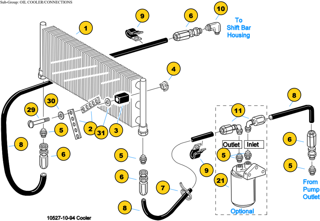
10527-10-94 Cooler
