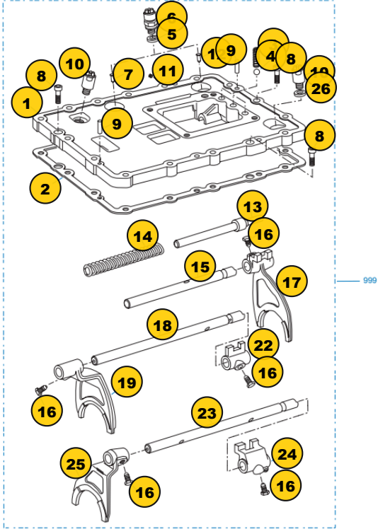
Group: BAR HOUSING ASSY
