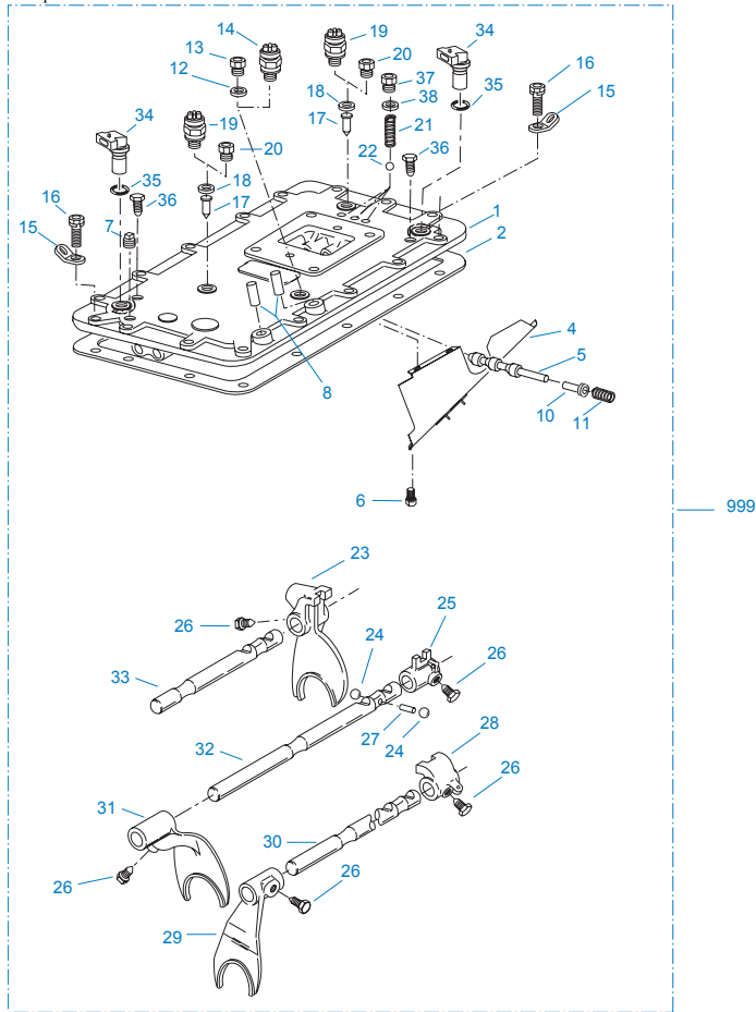
Group: SHIFT BAR HOUSING
