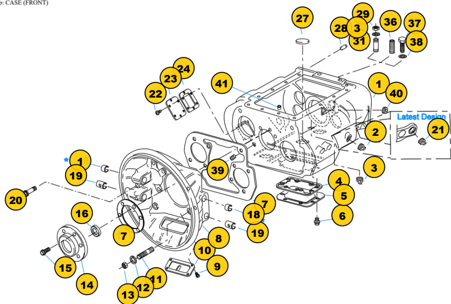
Group: CASE (FRONT)
