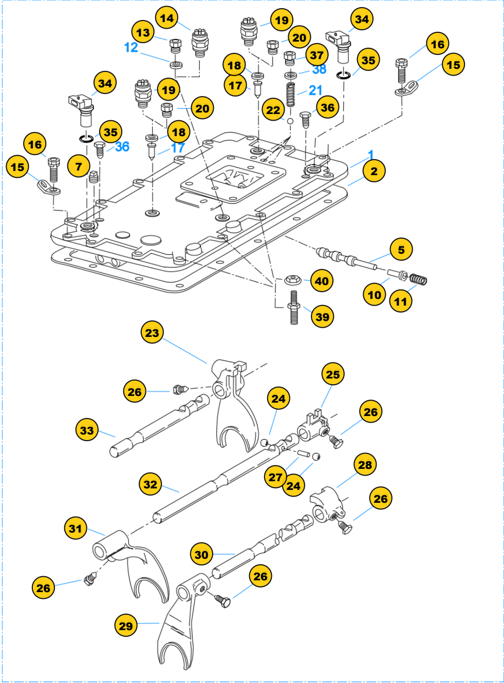
Group: SHIFT BAR HOUSING
