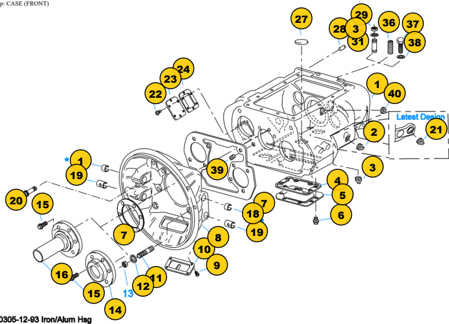
10305-12-93 Iron/Alum Hsg
