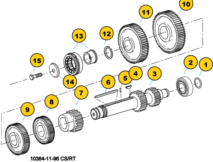
Group: COUNTERSHAFT ASSY
