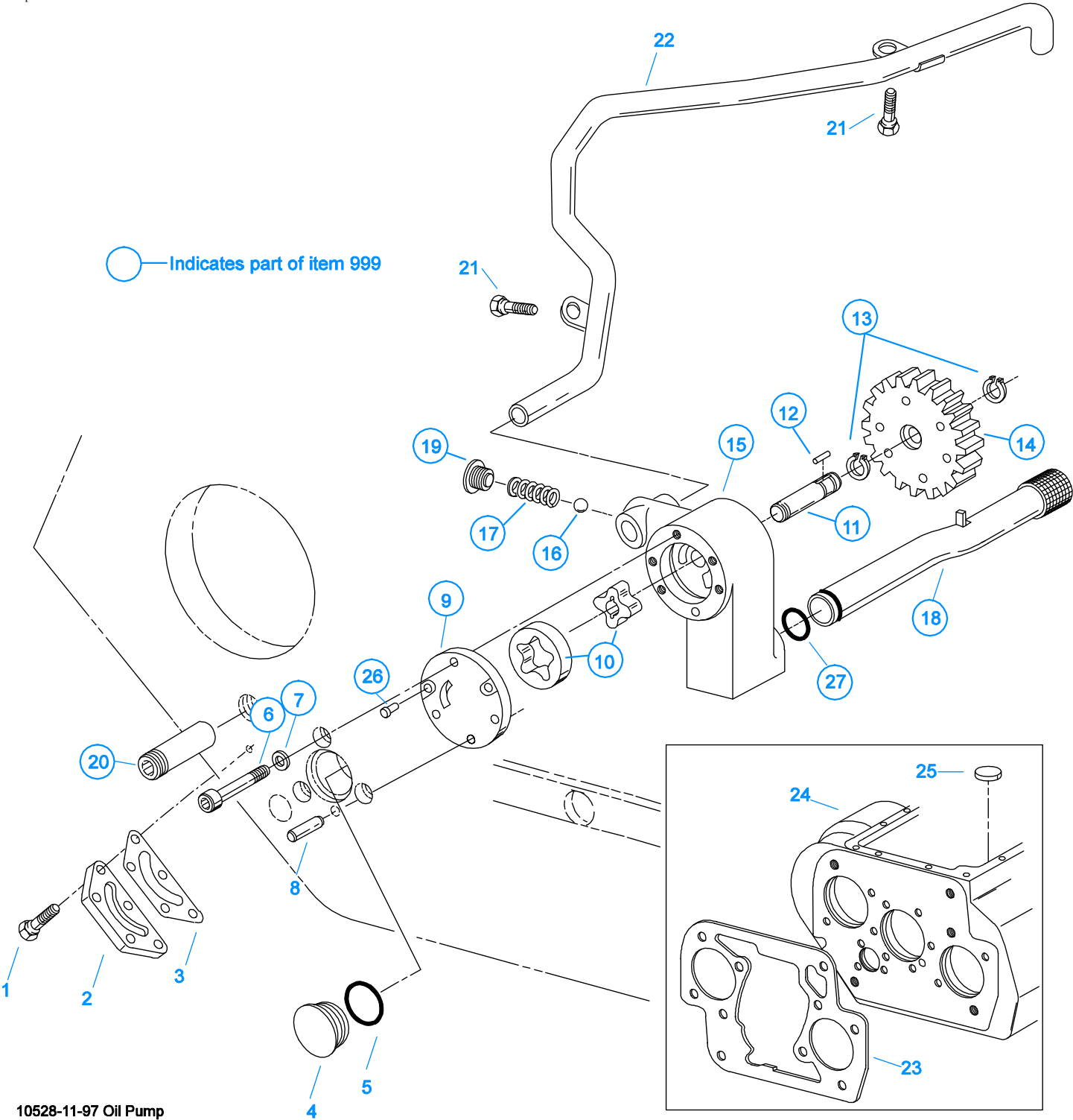
10528-11-97 Oil Pump
