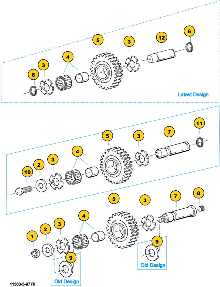
Group: REVERSE IDLER
