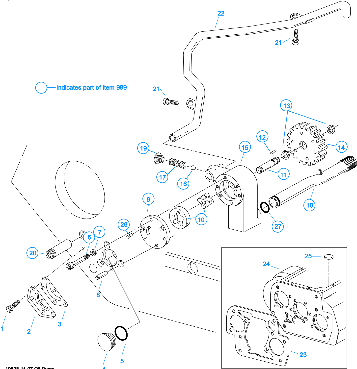
10528-11-97 Oil Pump
