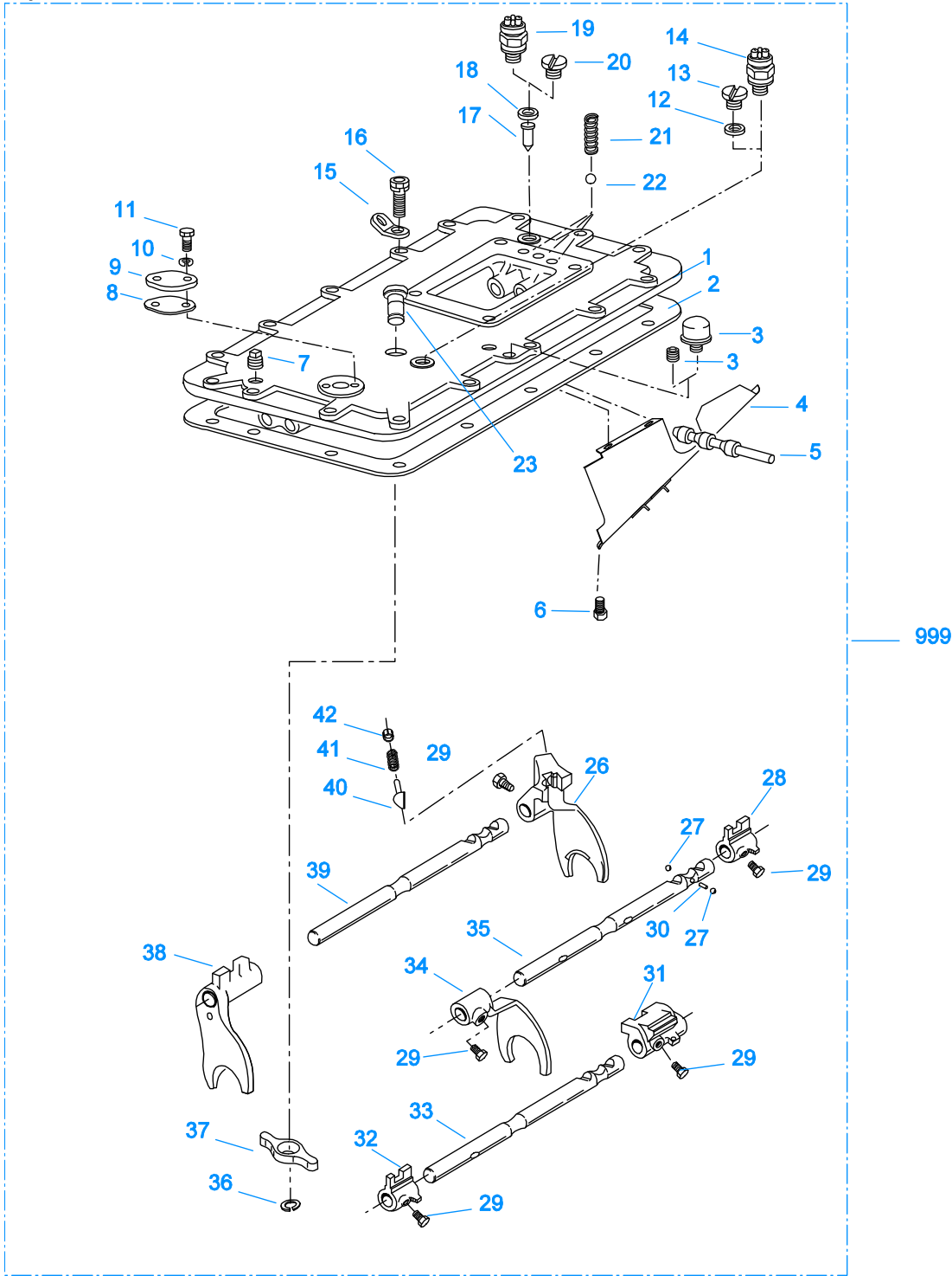
10244-11-96 X-Bar
