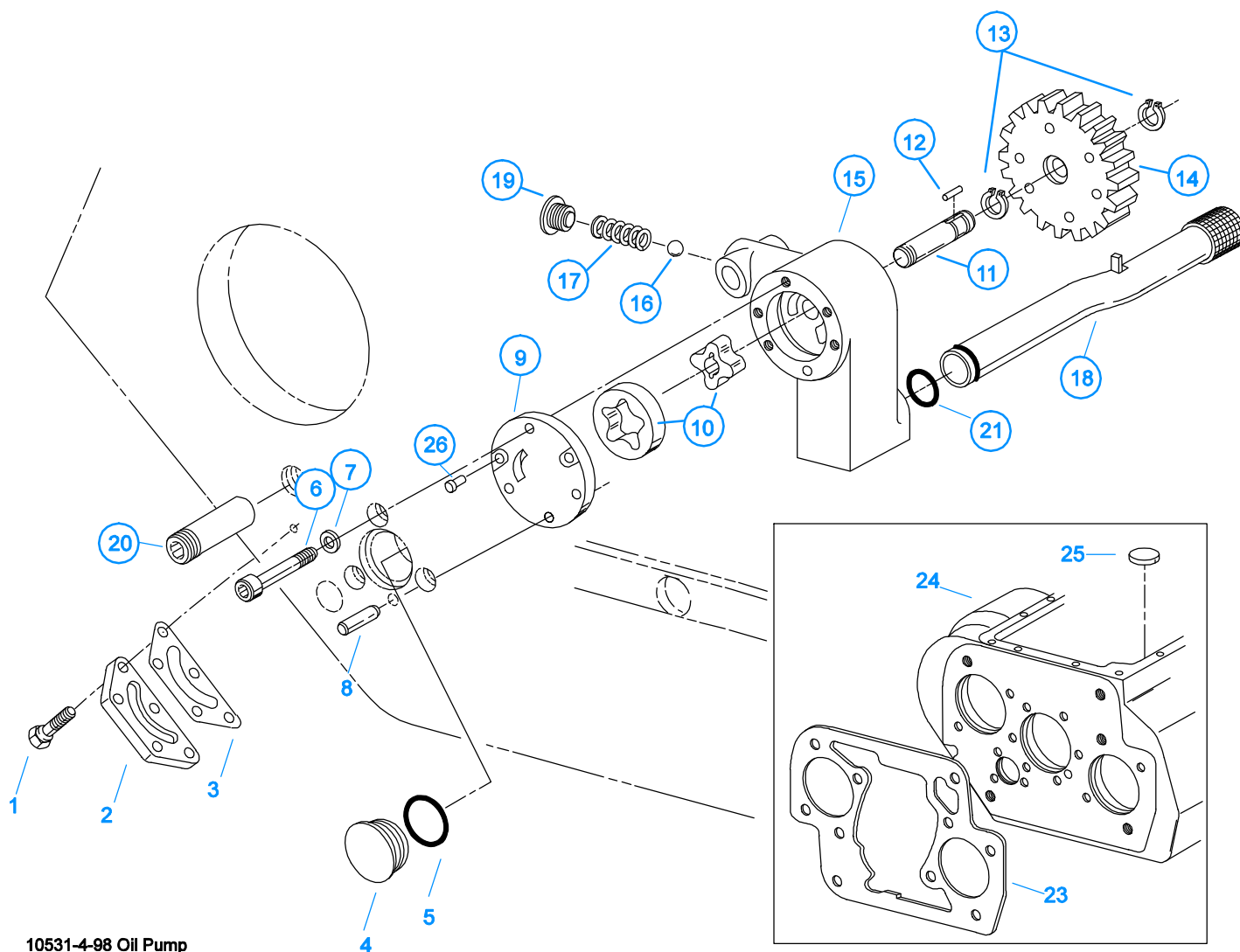
10531-4-98 Oil Pump
